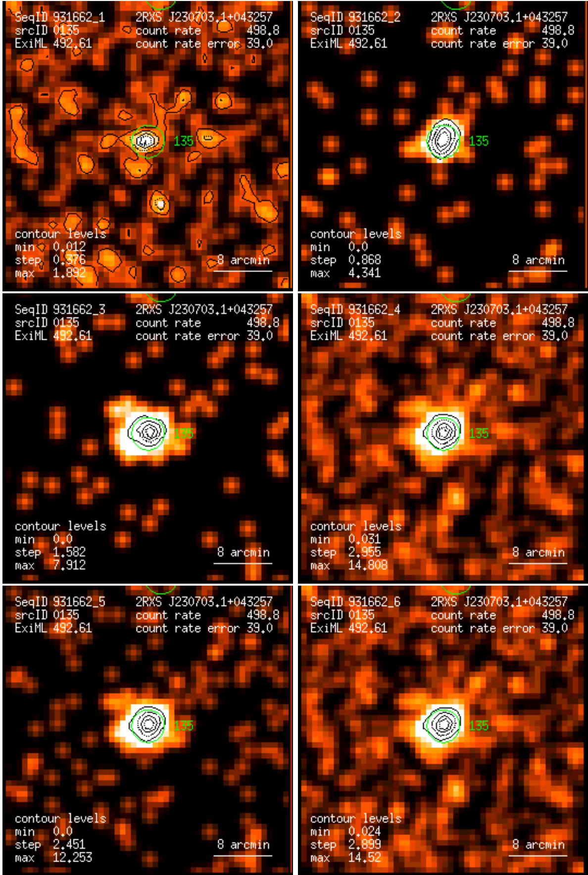
Figure 135: RASS 931662: detection 0135: band rate images, Gaussian filter: (1) PSPC channels 11 – 41, (2) 52 – 90, (3) 91 – 201, (4) 11 – 235, (5) 52 – 201, (6) 11 – 201. Broad band rates in counts/ks. Band rate contour levels in counts/ks/arcmin 2 .
