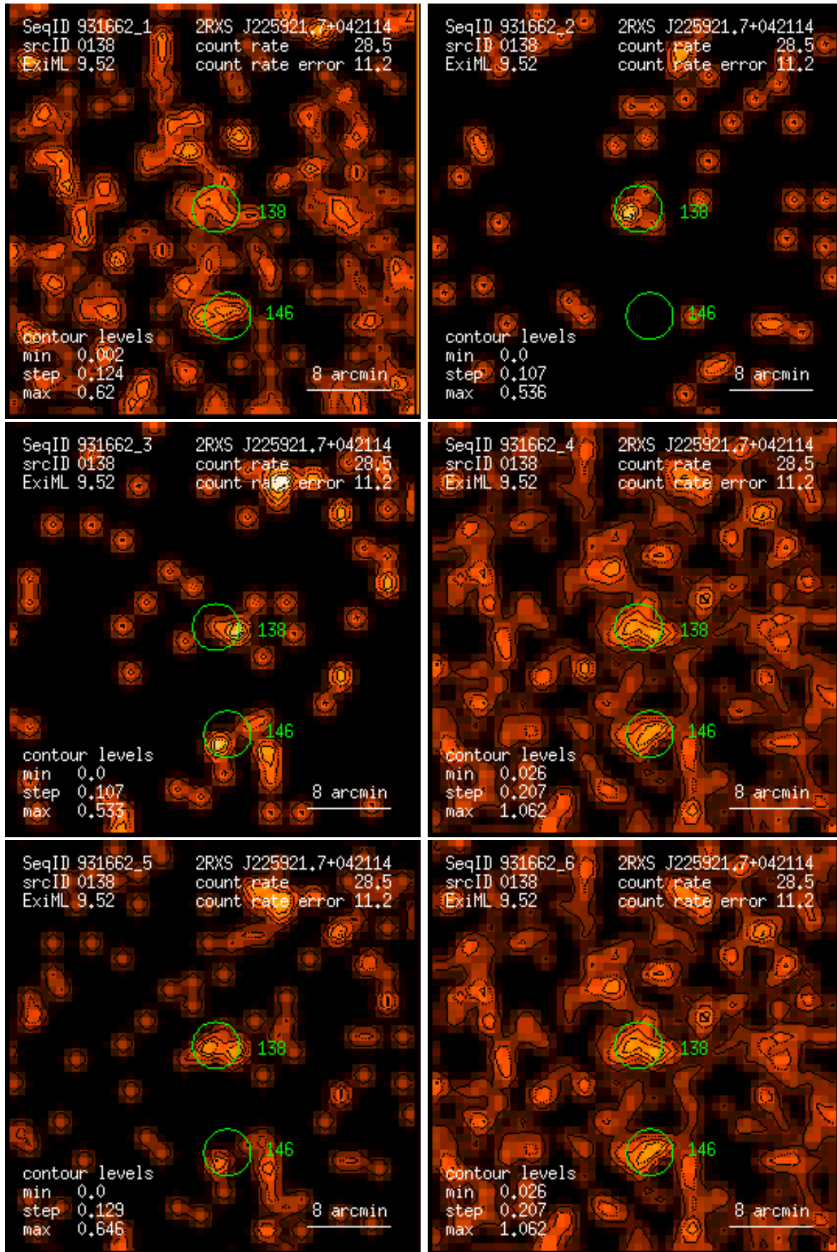
Figure 138: RASS 931662: detection 0138: band rate images, Gaussian filter: (1) PSPC channels 11 – 41, (2) 52 – 90, (3) 91 – 201, (4) 11 – 235, (5) 52 – 201, (6) 11 – 201. Broad band rates in counts/ks. Band rate contour levels in counts/ks/arcmin 2 .
