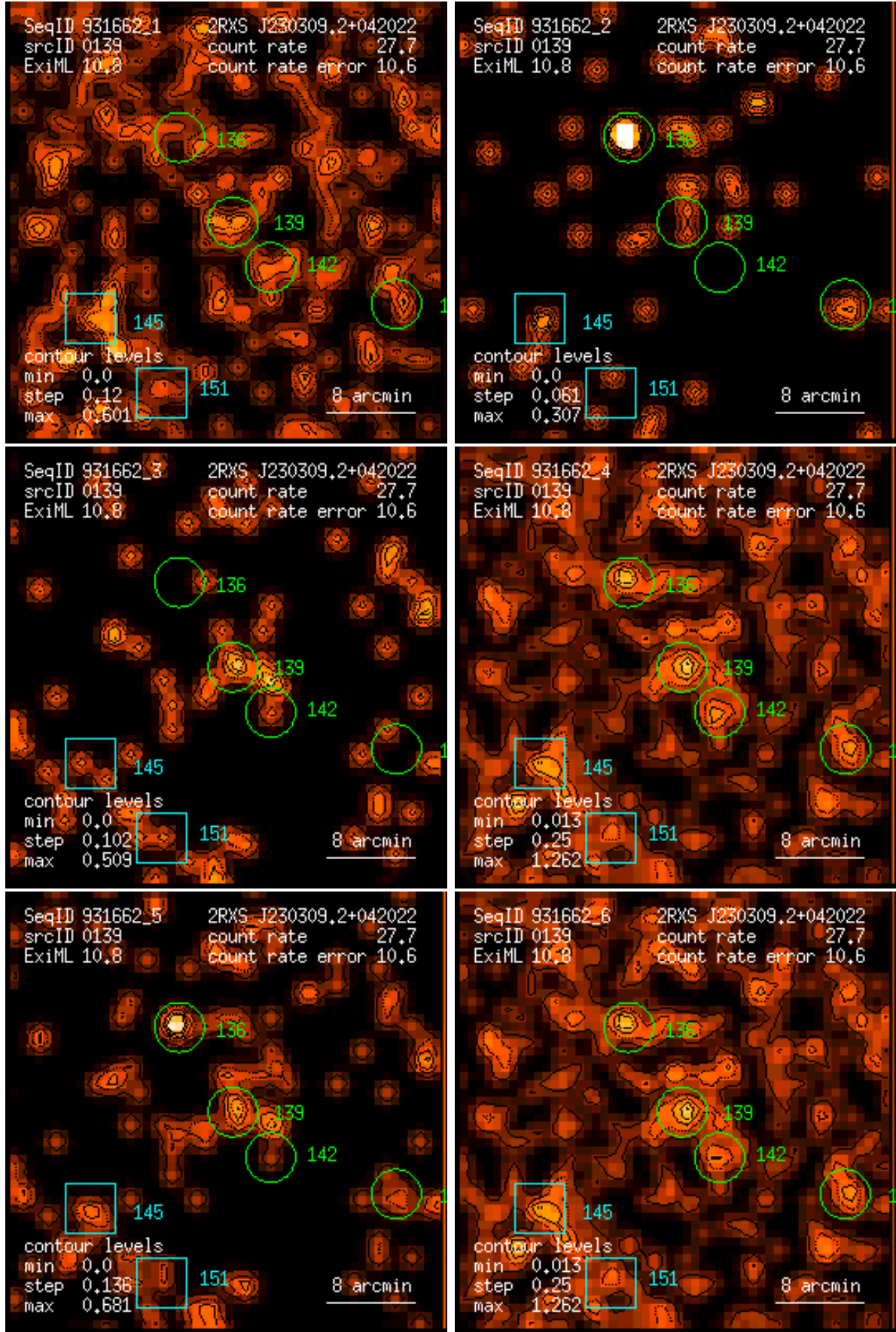
Figure 139: RASS 931662: detection 0139: band rate images, Gaussian filter: (1) PSPC channels 11 – 41, (2) 52 – 90, (3) 91 – 201, (4) 11 – 235, (5) 52 – 201, (6) 11 – 201. Broad band rates in counts/ks. Band rate contour levels in counts/ks/arcmin 2 .
