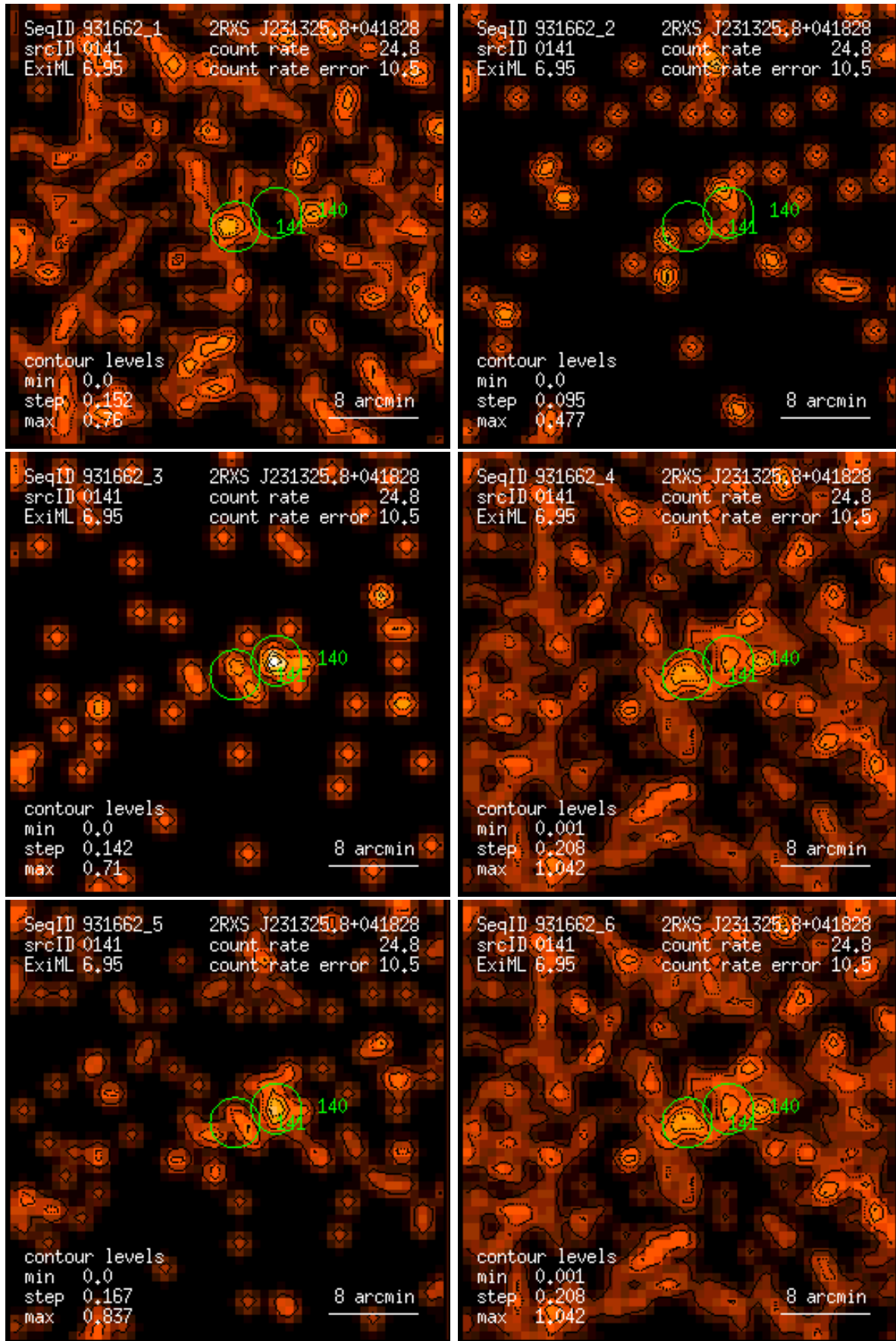
Figure 141: RASS 931662: detection 0141: band rate images, Gaussian filter: (1) PSPC channels 11 – 41, (2) 52 – 90, (3) 91 – 201, (4) 11 – 235, (5) 52 – 201, (6) 11 – 201. Broad band rates in counts/ks. Band rate contour levels in counts/ks/arcmin 2 .
