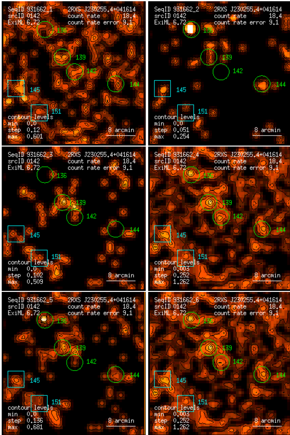
Figure 142: RASS 931662: detection 0142: band rate images, Gaussian filter: (1) PSPC channels 11 – 41, (2) 52 – 90, (3) 91 – 201, (4) 11 – 235, (5) 52 – 201, (6) 11 – 201. Broad band rates in counts/ks. Band rate contour levels in counts/ks/arcmin 2 .
