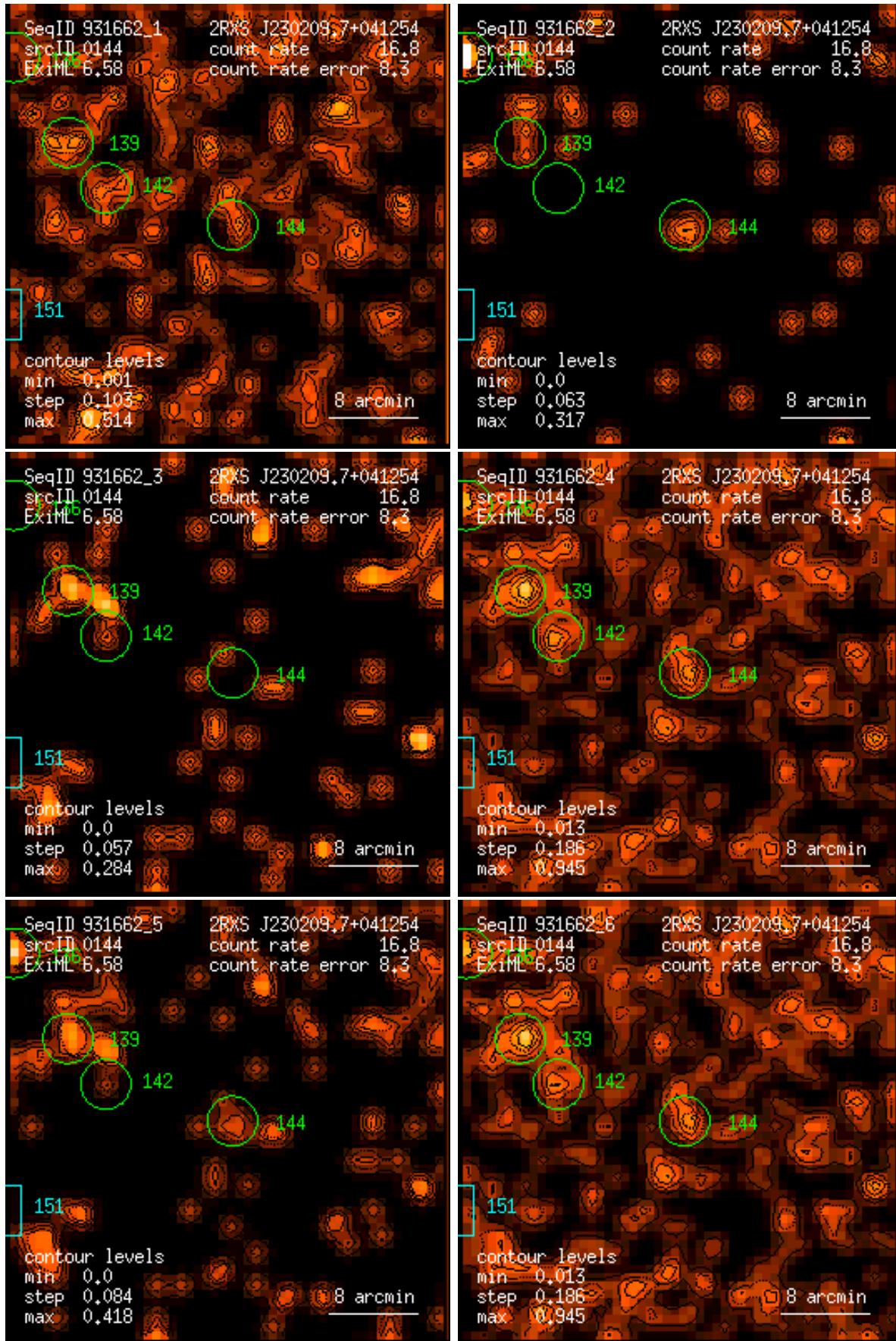
Figure 144: RASS 931662: detection 0144: band rate images, Gaussian filter: (1) PSPC channels 11 – 41, (2) 52 – 90, (3) 91 – 201, (4) 11 – 235, (5) 52 – 201, (6) 11 – 201. Broad band rates in counts/ks. Band rate contour levels in counts/ks/arcmin 2 .
