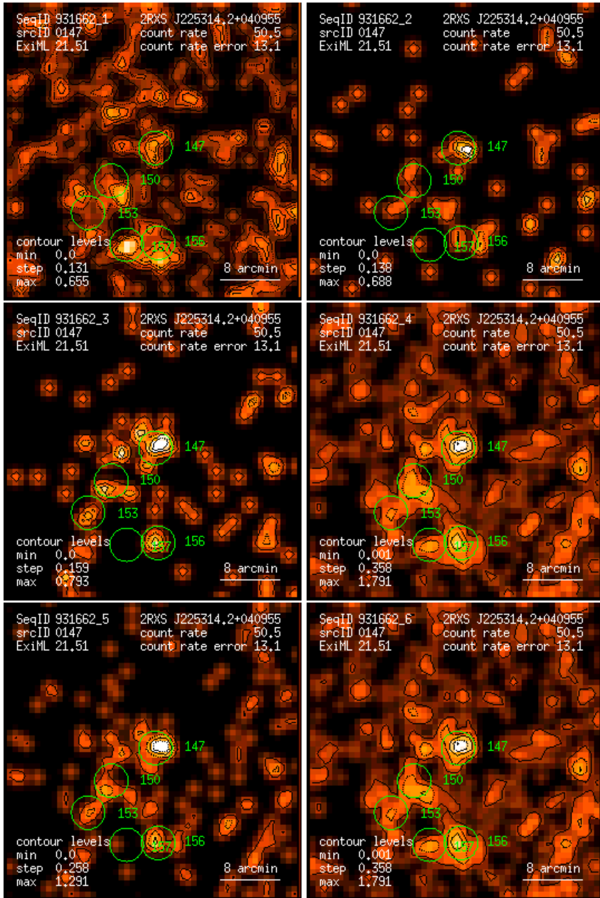
Figure 147: RASS 931662: detection 0147: band rate images, Gaussian filter: (1) PSPC channels 11 – 41, (2) 52 – 90, (3) 91 – 201, (4) 11 – 235, (5) 52 – 201, (6) 11 – 201. Broad band rates in counts/ks. Band rate contour levels in counts/ks/arcmin 2 .
