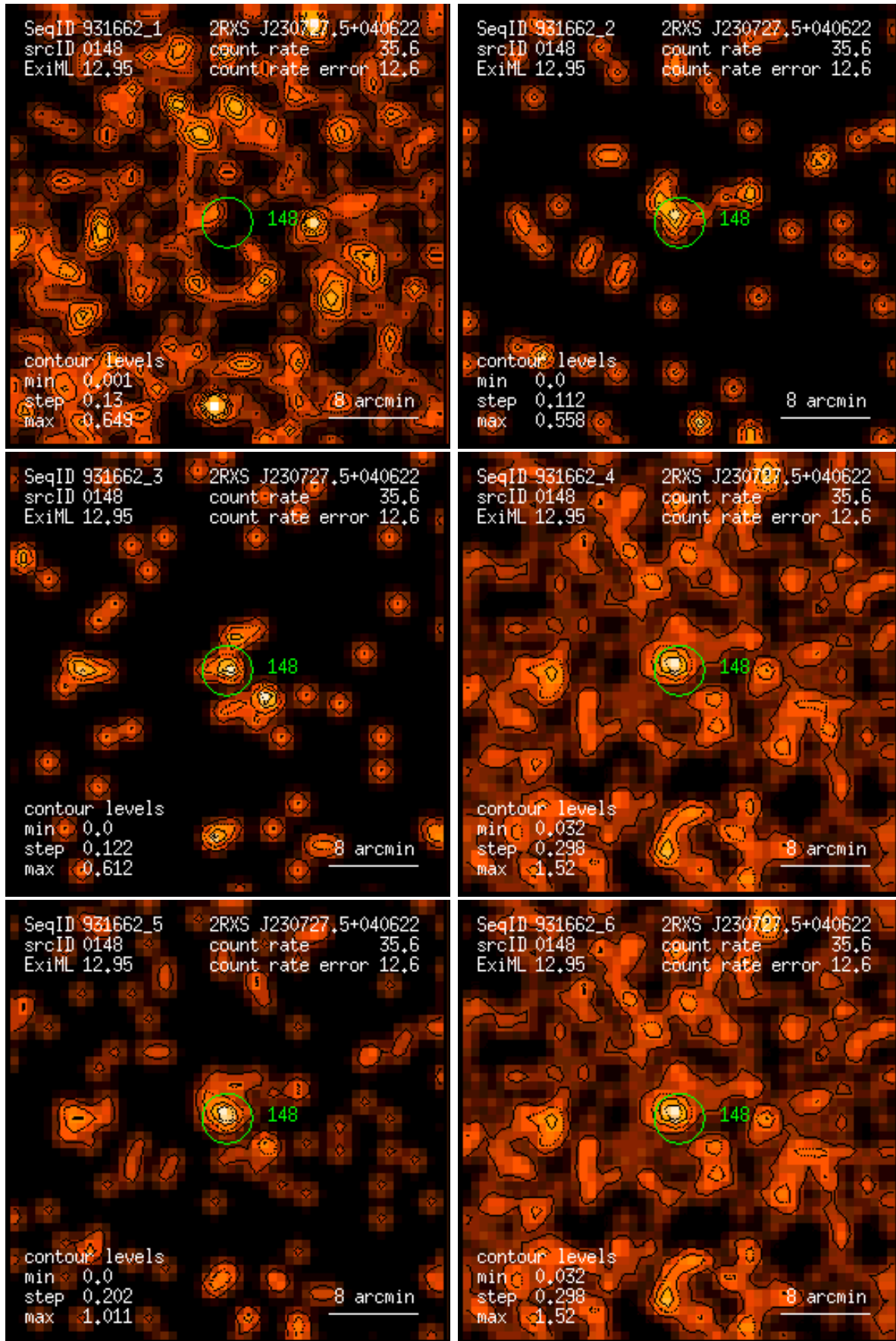
Figure 148: RASS 931662: detection 0148: band rate images, Gaussian filter: (1) PSPC channels 11 – 41, (2) 52 – 90, (3) 91 – 201, (4) 11 – 235, (5) 52 – 201, (6) 11 – 201. Broad band rates in counts/ks. Band rate contour levels in counts/ks/arcmin 2 .
