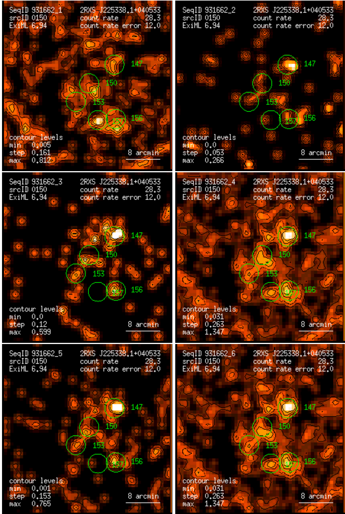
Figure 150: RASS 931662: detection 0150: band rate images, Gaussian filter: (1) PSPC channels 11 – 41, (2) 52 – 90, (3) 91 – 201, (4) 11 – 235, (5) 52 – 201, (6) 11 – 201. Broad band rates in counts/ks. Band rate contour levels in counts/ks/arcmin 2 .
