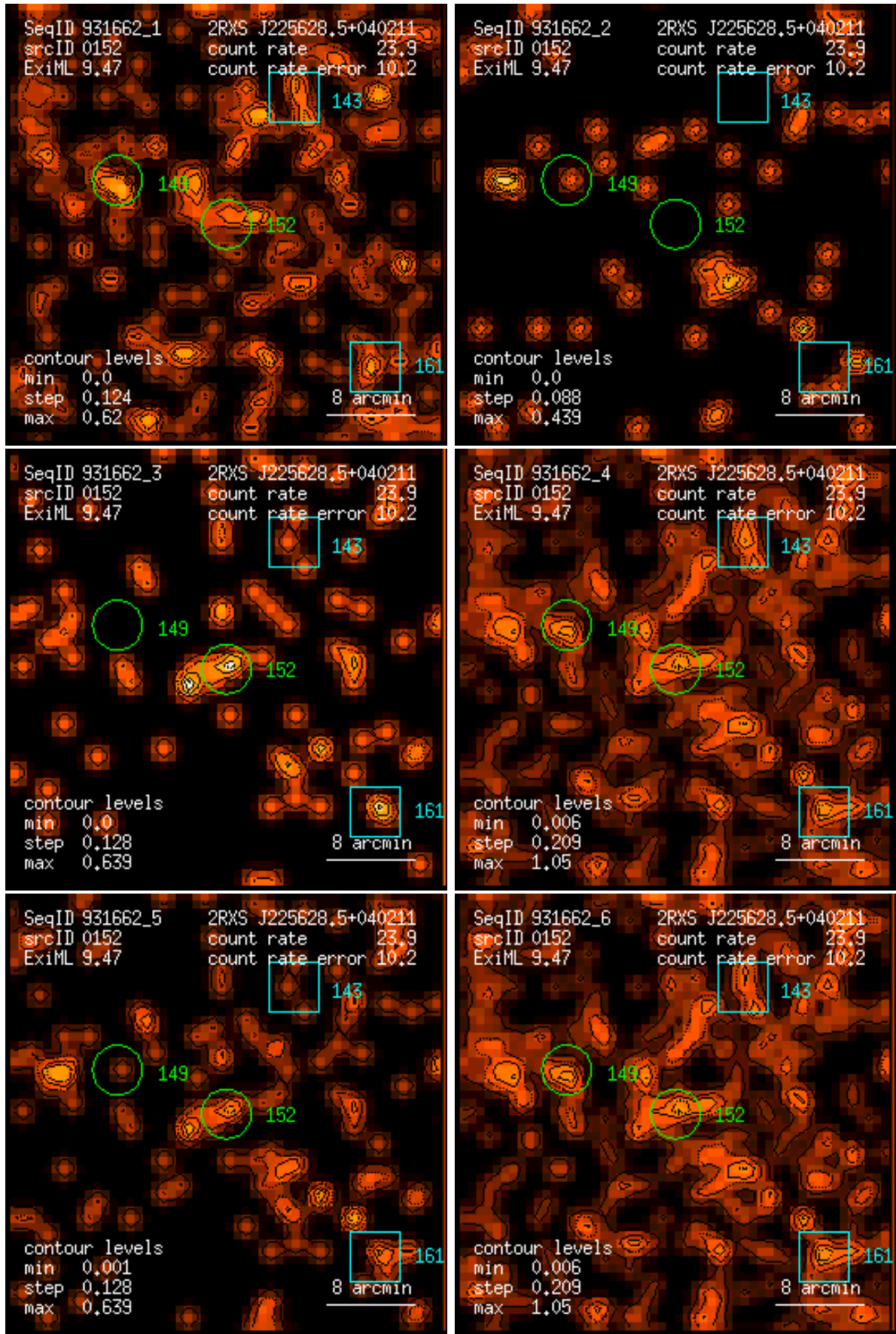
Figure 152: RASS 931662: detection 0152: band rate images, Gaussian filter: (1) PSPC channels 11 – 41, (2) 52 – 90, (3) 91 – 201, (4) 11 – 235, (5) 52 – 201, (6) 11 – 201. Broad band rates in counts/ks. Band rate contour levels in counts/ks/arcmin 2 .
