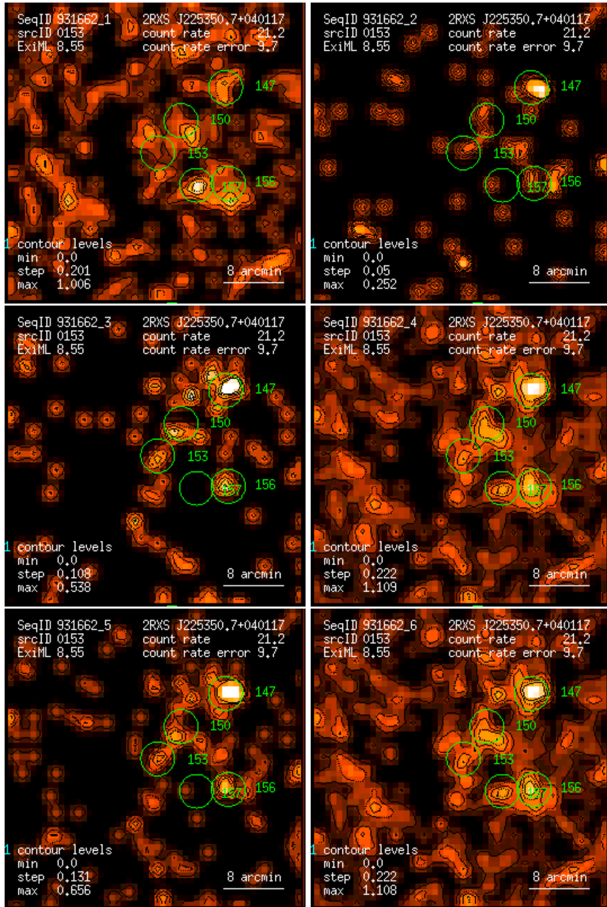
Figure 153: RASS 931662: detection 0153: band rate images, Gaussian filter: (1) PSPC channels 11 – 41, (2) 52 – 90, (3) 91 – 201, (4) 11 – 235, (5) 52 – 201, (6) 11 – 201. Broad band rates in counts/ks. Band rate contour levels in counts/ks/arcmin 2 .
