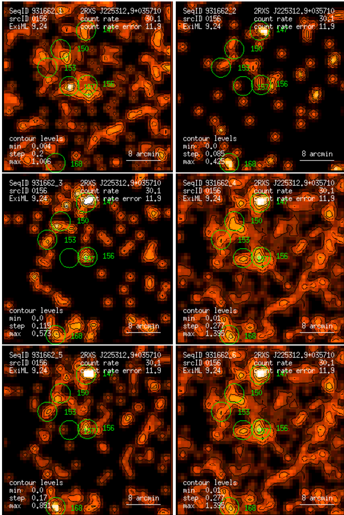
Figure 156: RASS 931662: detection 0156: band rate images, Gaussian filter: (1) PSPC channels 11 – 41, (2) 52 – 90, (3) 91 – 201, (4) 11 – 235, (5) 52 – 201, (6) 11 – 201. Broad band rates in counts/ks. Band rate contour levels in counts/ks/arcmin 2 .
