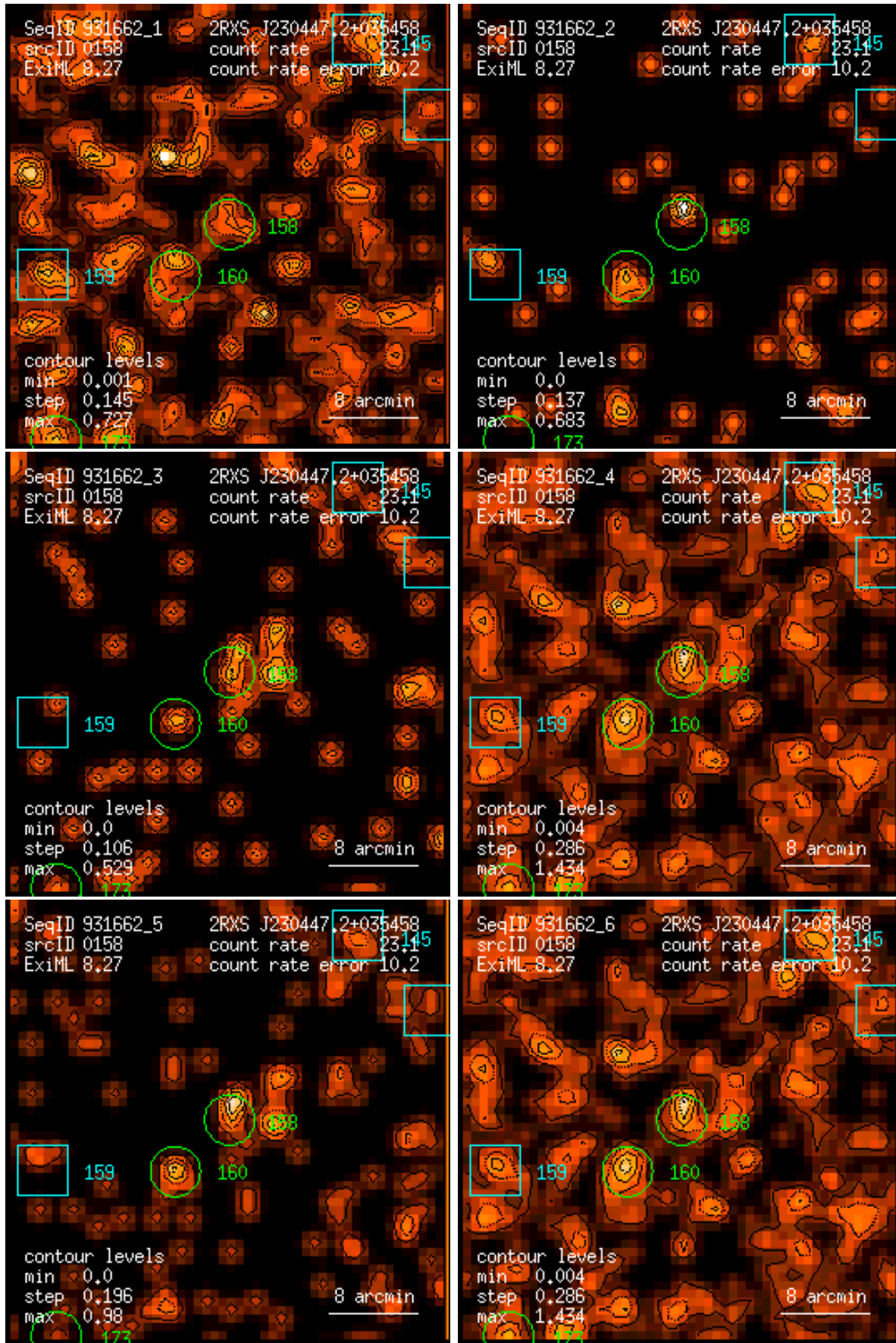
Figure 158: RASS 931662: detection 0158: band rate images, Gaussian filter: (1) PSPC channels 11 – 41, (2) 52 – 90, (3) 91 – 201, (4) 11 – 235, (5) 52 – 201, (6) 11 – 201. Broad band rates in counts/ks. Band rate contour levels in counts/ks/arcmin 2 .
