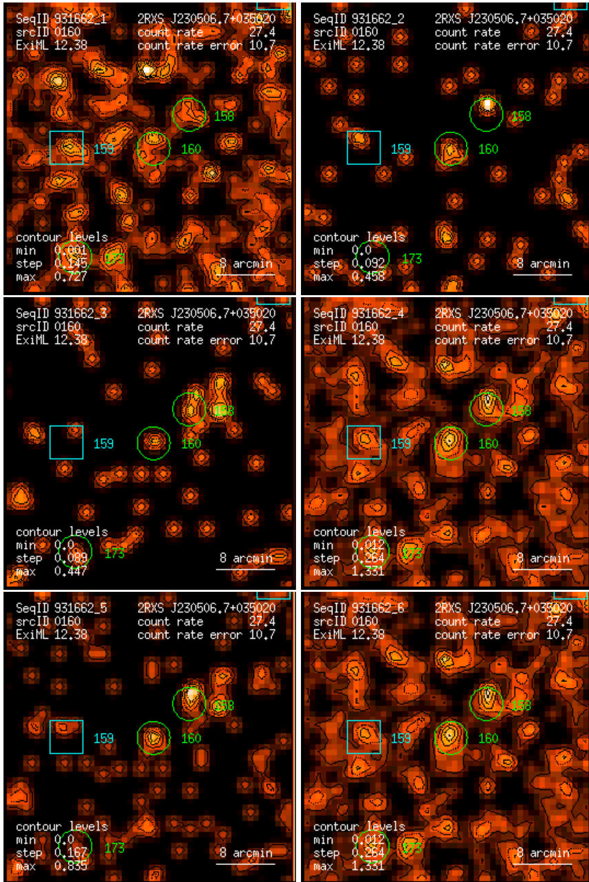
Figure 160: RASS 931662: detection 0160: band rate images, Gaussian filter: (1) PSPC channels 11 – 41, (2) 52 – 90, (3) 91 – 201, (4) 11 – 235, (5) 52 – 201, (6) 11 – 201. Broad band rates in counts/ks. Band rate contour levels in counts/ks/arcmin 2 .
