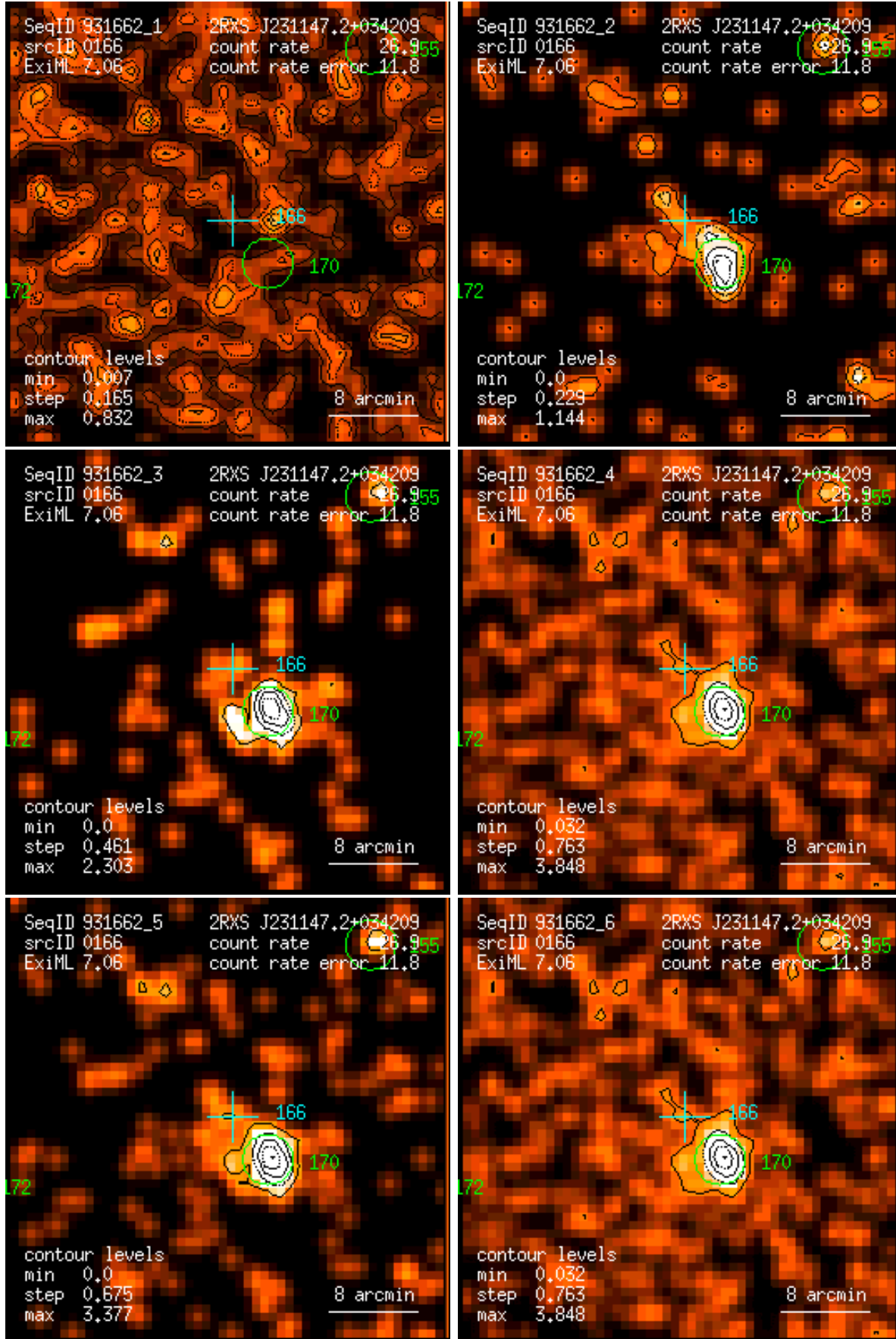
Figure 166: RASS 931662: detection 0166: band rate images, Gaussian filter: (1) PSPC channels 11 – 41, (2) 52 – 90, (3) 91 – 201, (4) 11 – 235, (5) 52 – 201, (6) 11 – 201. Broad band rates in counts/ks. Band rate contour levels in counts/ks/arcmin 2 .
