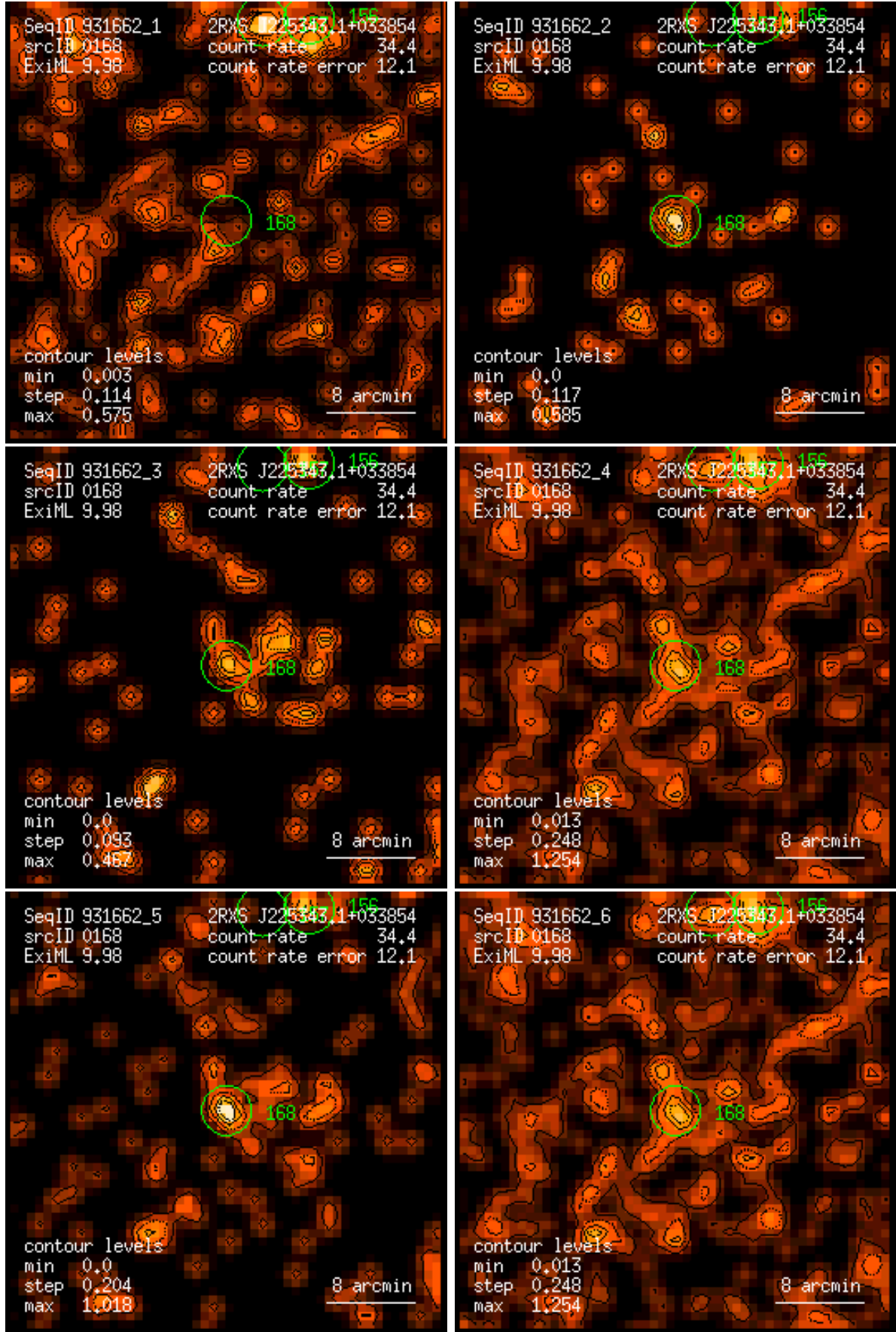
Figure 168: RASS 931662: detection 0168: band rate images, Gaussian filter: (1) PSPC channels 11 – 41, (2) 52 – 90, (3) 91 – 201, (4) 11 – 235, (5) 52 – 201, (6) 11 – 201. Broad band rates in counts/ks. Band rate contour levels in counts/ks/arcmin 2 .
