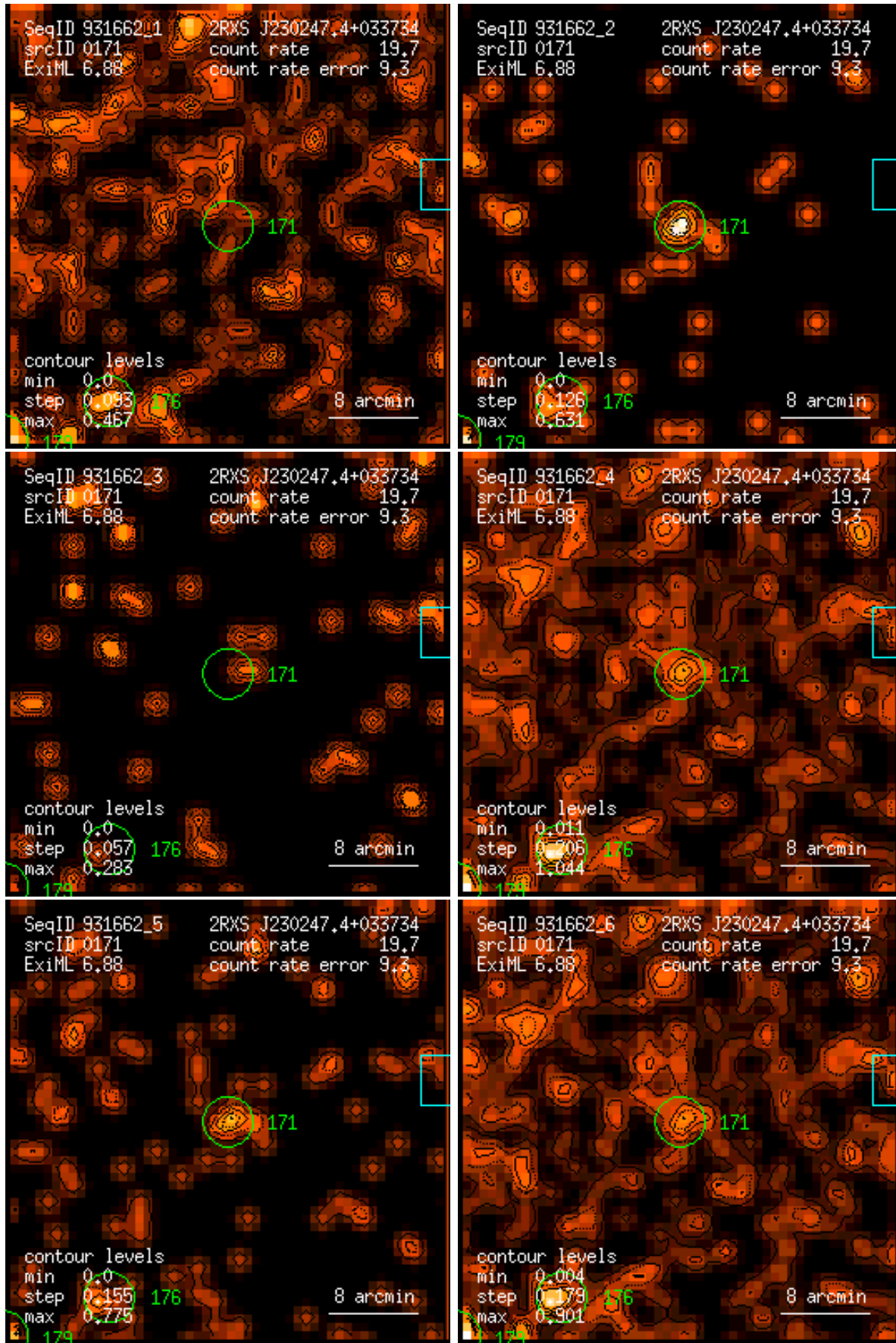
Figure 171: RASS 931662: detection 0171: band rate images, Gaussian filter: (1) PSPC channels 11 – 41, (2) 52 – 90, (3) 91 – 201, (4) 11 – 235, (5) 52 – 201, (6) 11 – 201. Broad band rates in counts/ks. Band rate contour levels in counts/ks/arcmin 2 .
