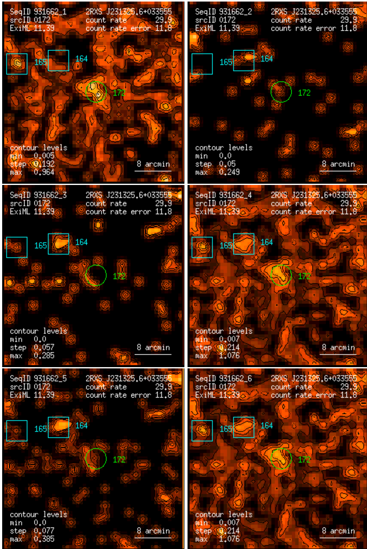
Figure 172: RASS 931662: detection 0172: band rate images, Gaussian filter: (1) PSPC channels 11 – 41, (2) 52 – 90, (3) 91 – 201, (4) 11 – 235, (5) 52 – 201, (6) 11 – 201. Broad band rates in counts/ks. Band rate contour levels in counts/ks/arcmin 2 .
