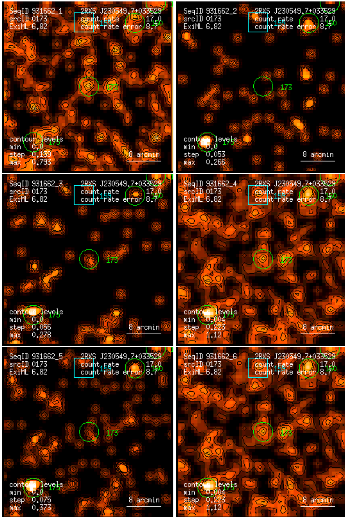
Figure 173: RASS 931662: detection 0173: band rate images, Gaussian filter: (1) PSPC channels 11 – 41, (2) 52 – 90, (3) 91 – 201, (4) 11 – 235, (5) 52 – 201, (6) 11 – 201. Broad band rates in counts/ks. Band rate contour levels in counts/ks/arcmin 2 .
