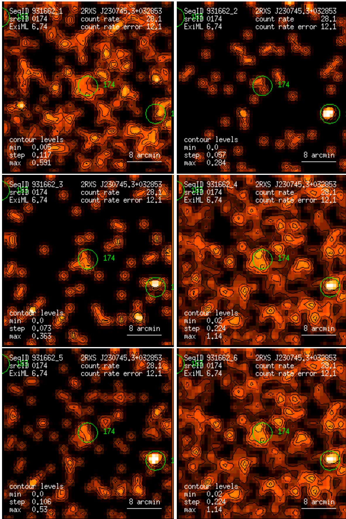
Figure 174: RASS 931662: detection 0174: band rate images, Gaussian filter: (1) PSPC channels 11 – 41, (2) 52 – 90, (3) 91 – 201, (4) 11 – 235, (5) 52 – 201, (6) 11 – 201. Broad band rates in counts/ks. Band rate contour levels in counts/ks/arcmin 2 .
