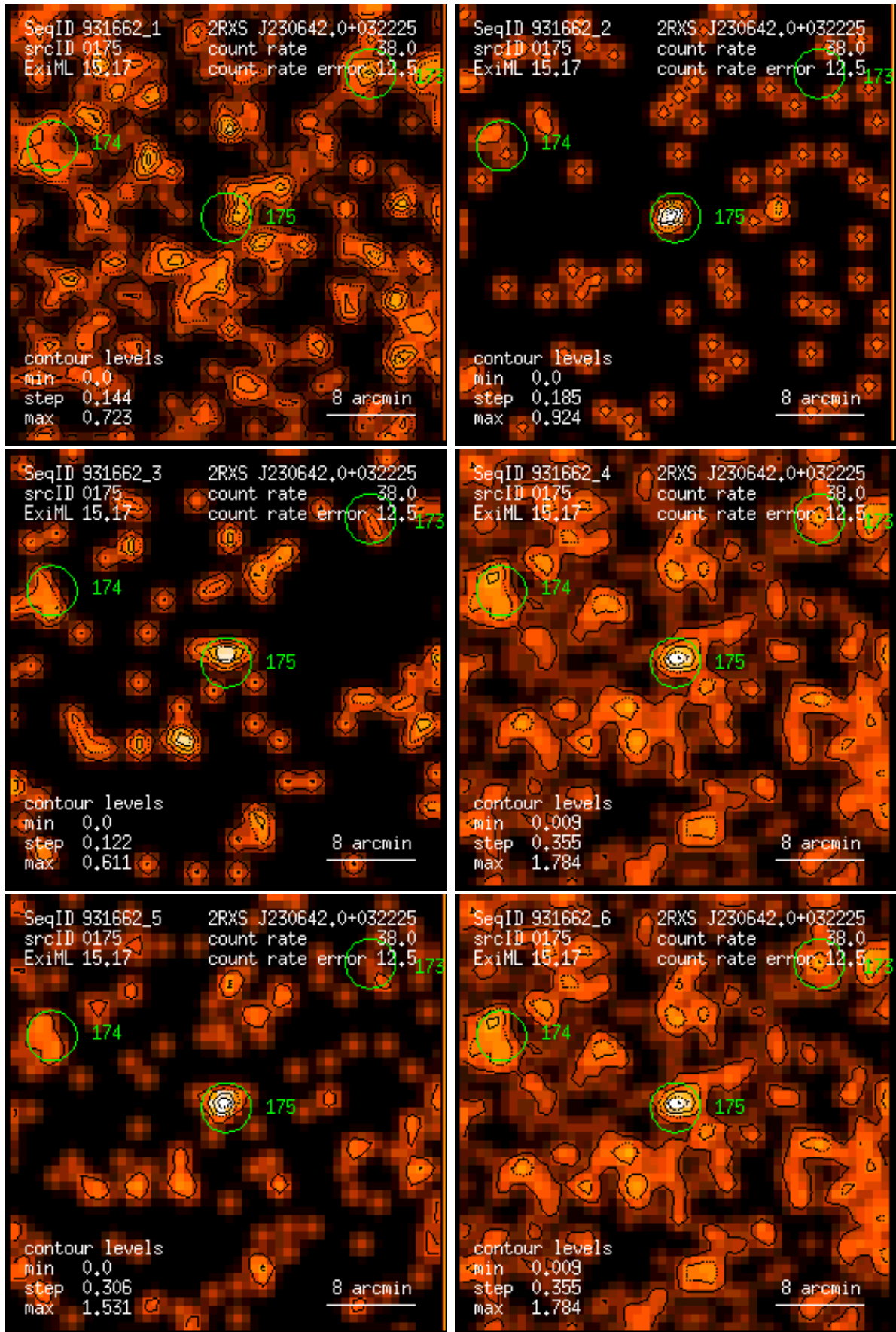
Figure 175: RASS 931662: detection 0175: band rate images, Gaussian filter: (1) PSPC channels 11 – 41, (2) 52 – 90, (3) 91 – 201, (4) 11 – 235, (5) 52 – 201, (6) 11 – 201. Broad band rates in counts/ks. Band rate contour levels in counts/ks/arcmin 2 .
