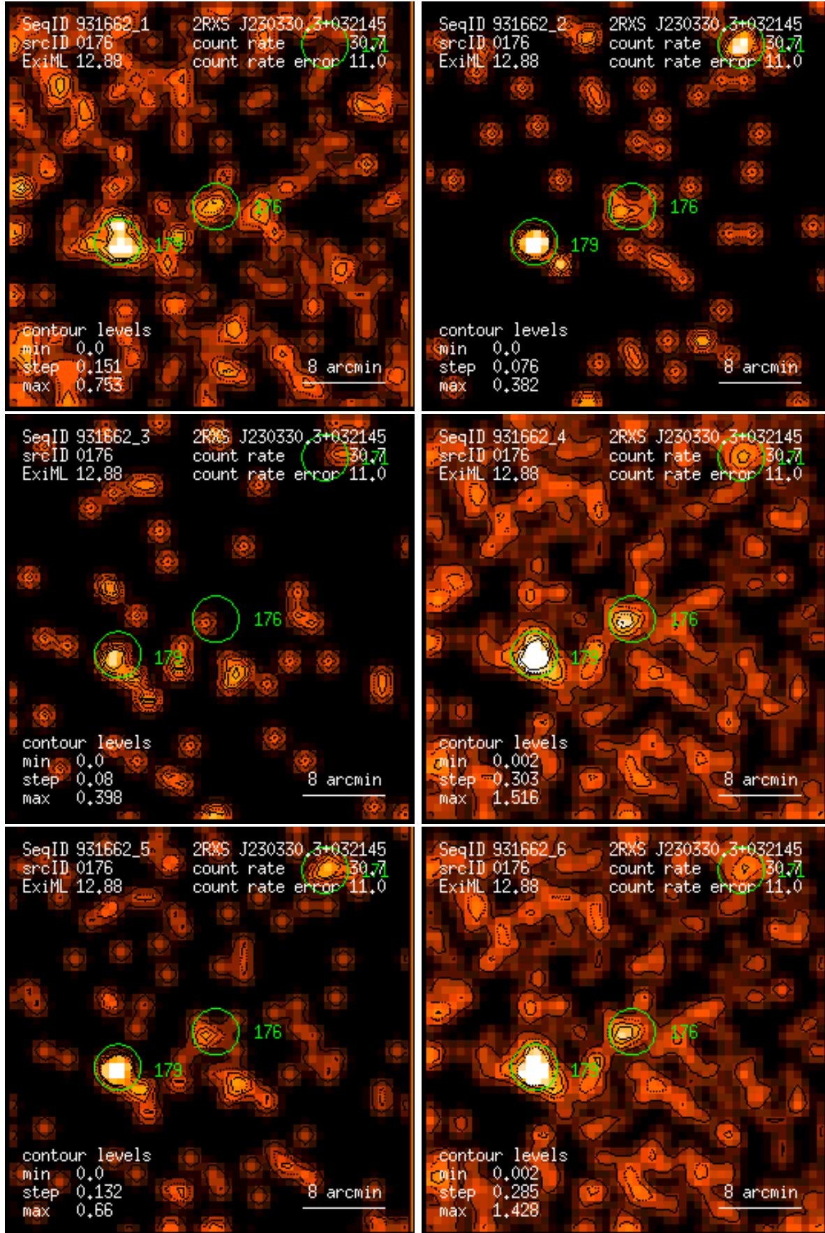
Figure 176: RASS 931662: detection 0176: band rate images, Gaussian filter: (1) PSPC channels 11 – 41, (2) 52 – 90, (3) 91 – 201, (4) 11 – 235, (5) 52 – 201, (6) 11 – 201. Broad band rates in counts/ks. Band rate contour levels in counts/ks/arcmin 2 .
