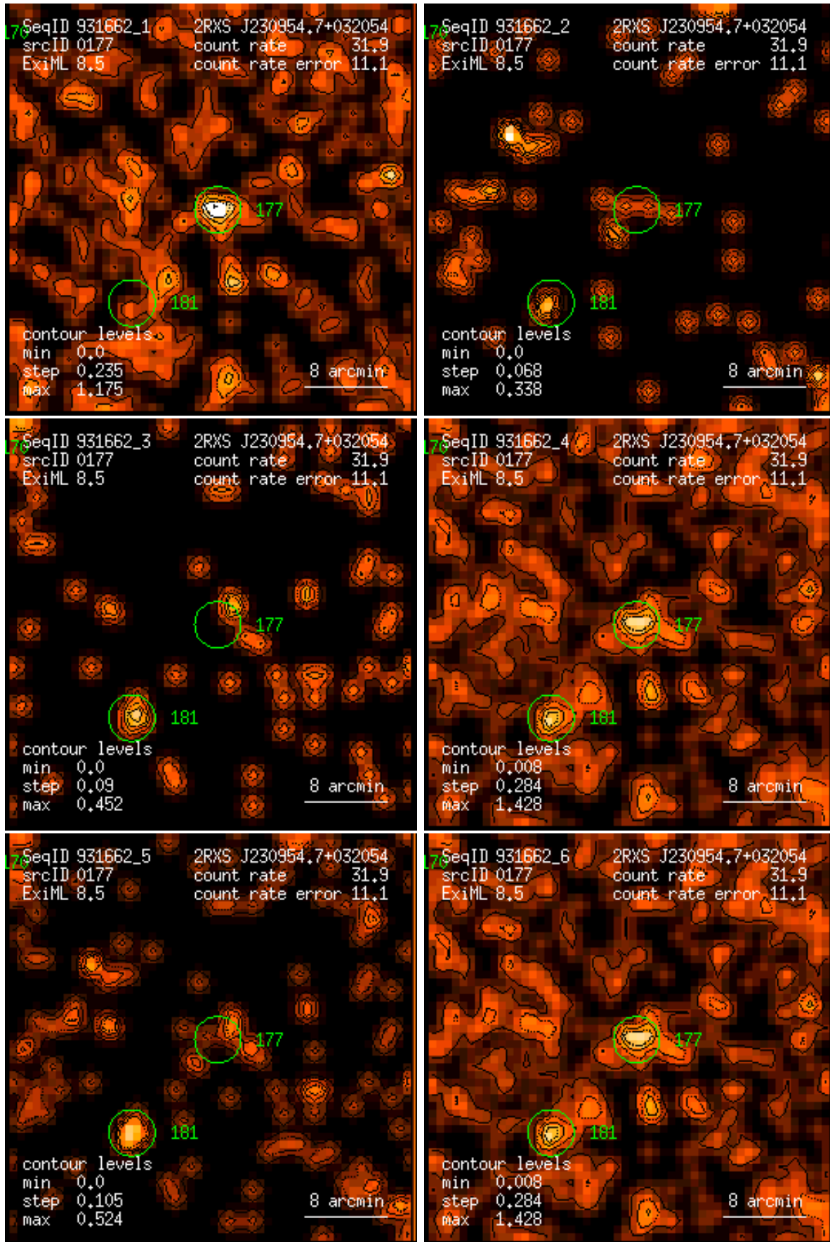
Figure 177: RASS 931662: detection 0177: band rate images, Gaussian filter: (1) PSPC channels 11 – 41, (2) 52 – 90, (3) 91 – 201, (4) 11 – 235, (5) 52 – 201, (6) 11 – 201. Broad band rates in counts/ks. Band rate contour levels in counts/ks/arcmin 2 .
