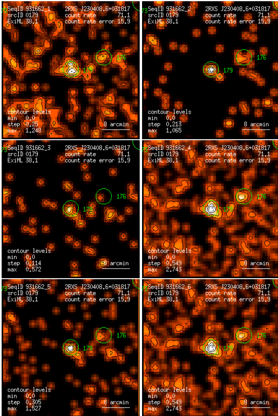
Figure 179: RASS 931662: detection 0179: band rate images, Gaussian filter: (1) PSPC channels 11 – 41, (2) 52 – 90, (3) 91 – 201, (4) 11 – 235, (5) 52 – 201, (6) 11 – 201. Broad band rates in counts/ks. Band rate contour levels in counts/ks/arcmin 2 .
