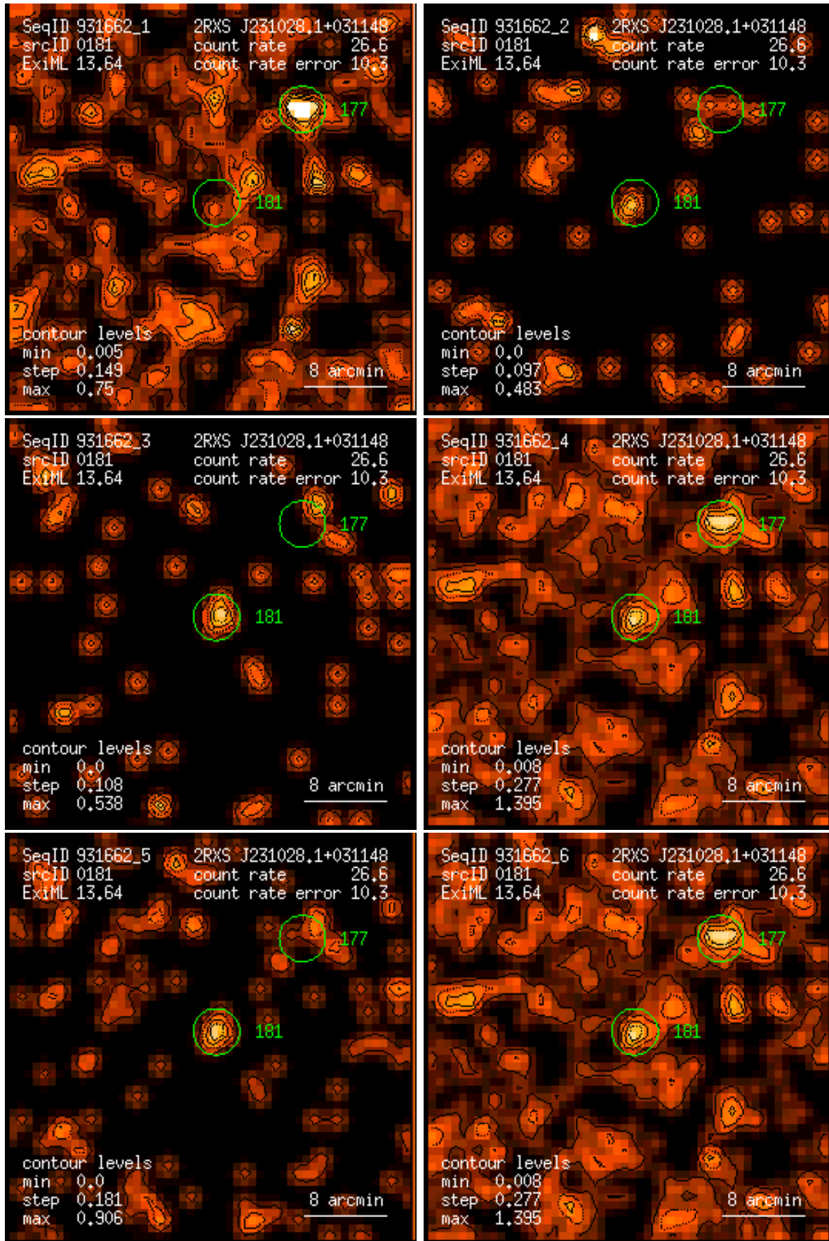
Figure 181: RASS 931662: detection 0181: band rate images, Gaussian filter: (1) PSPC channels 11 – 41, (2) 52 – 90, (3) 91 – 201, (4) 11 – 235, (5) 52 – 201, (6) 11 – 201. Broad band rates in counts/ks. Band rate contour levels in counts/ks/arcmin 2 .
