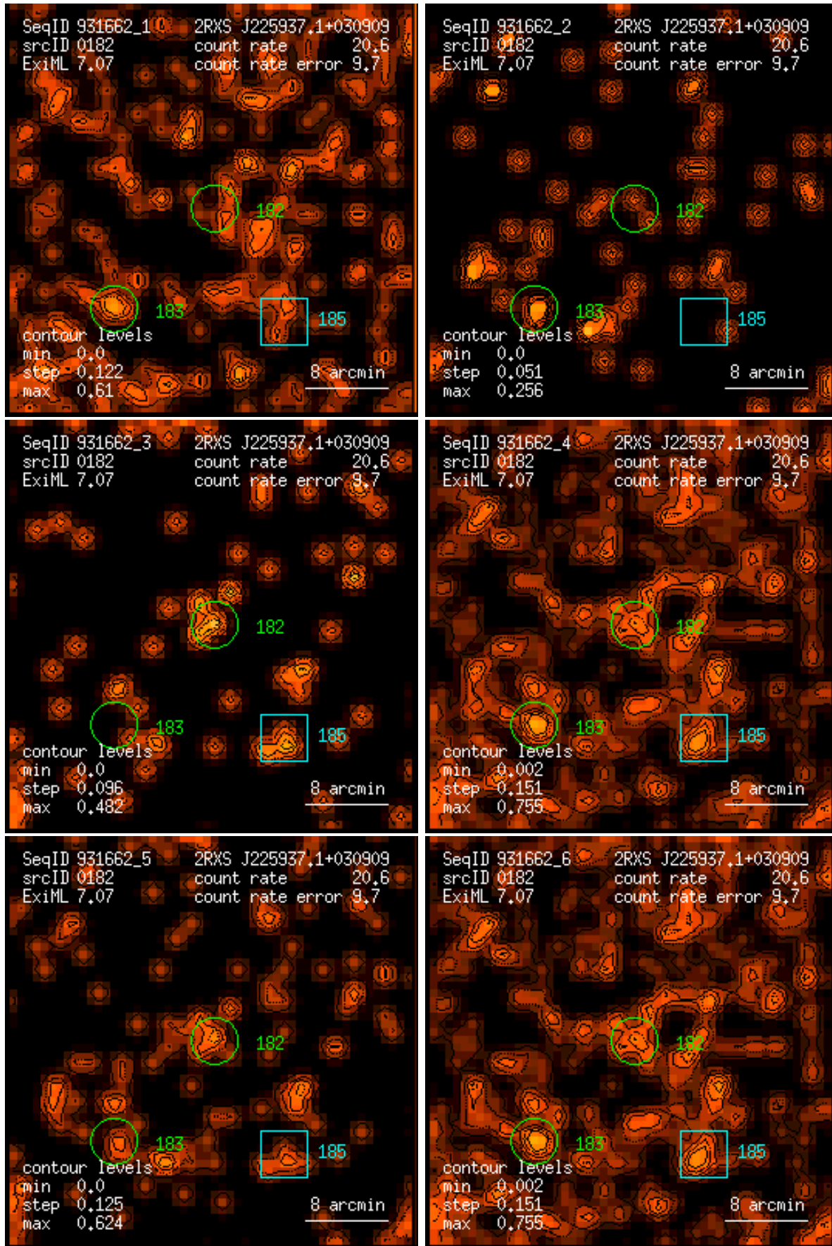
Figure 182: RASS 931662: detection 0182: band rate images, Gaussian filter: (1) PSPC channels 11 – 41, (2) 52 – 90, (3) 91 – 201, (4) 11 – 235, (5) 52 – 201, (6) 11 – 201. Broad band rates in counts/ks. Band rate contour levels in counts/ks/arcmin 2 .
