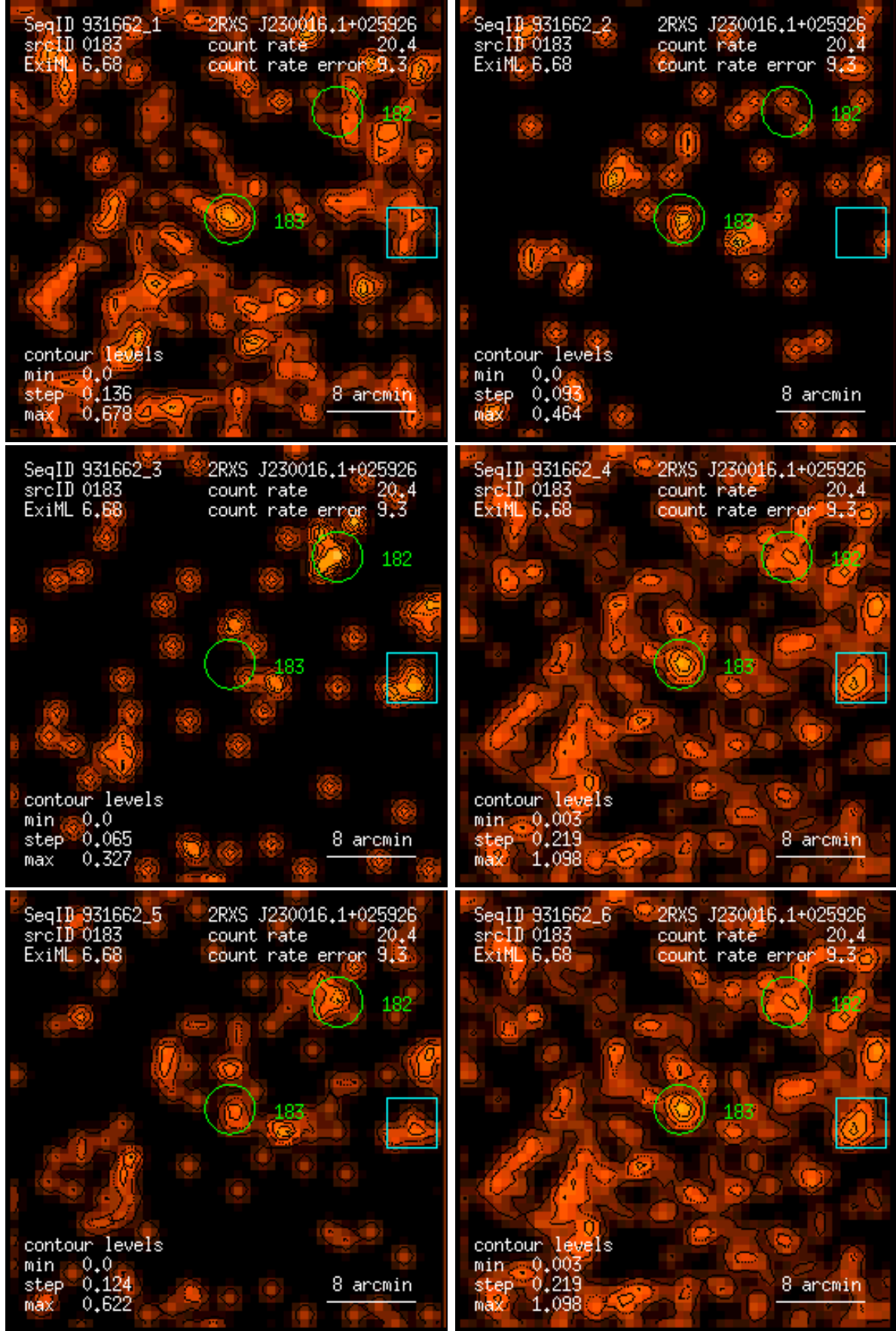
Figure 183: RASS 931662: detection 0183: band rate images, Gaussian filter: (1) PSPC channels 11 – 41, (2) 52 – 90, (3) 91 – 201, (4) 11 – 235, (5) 52 – 201, (6) 11 – 201. Broad band rates in counts/ks. Band rate contour levels in counts/ks/arcmin 2 .
