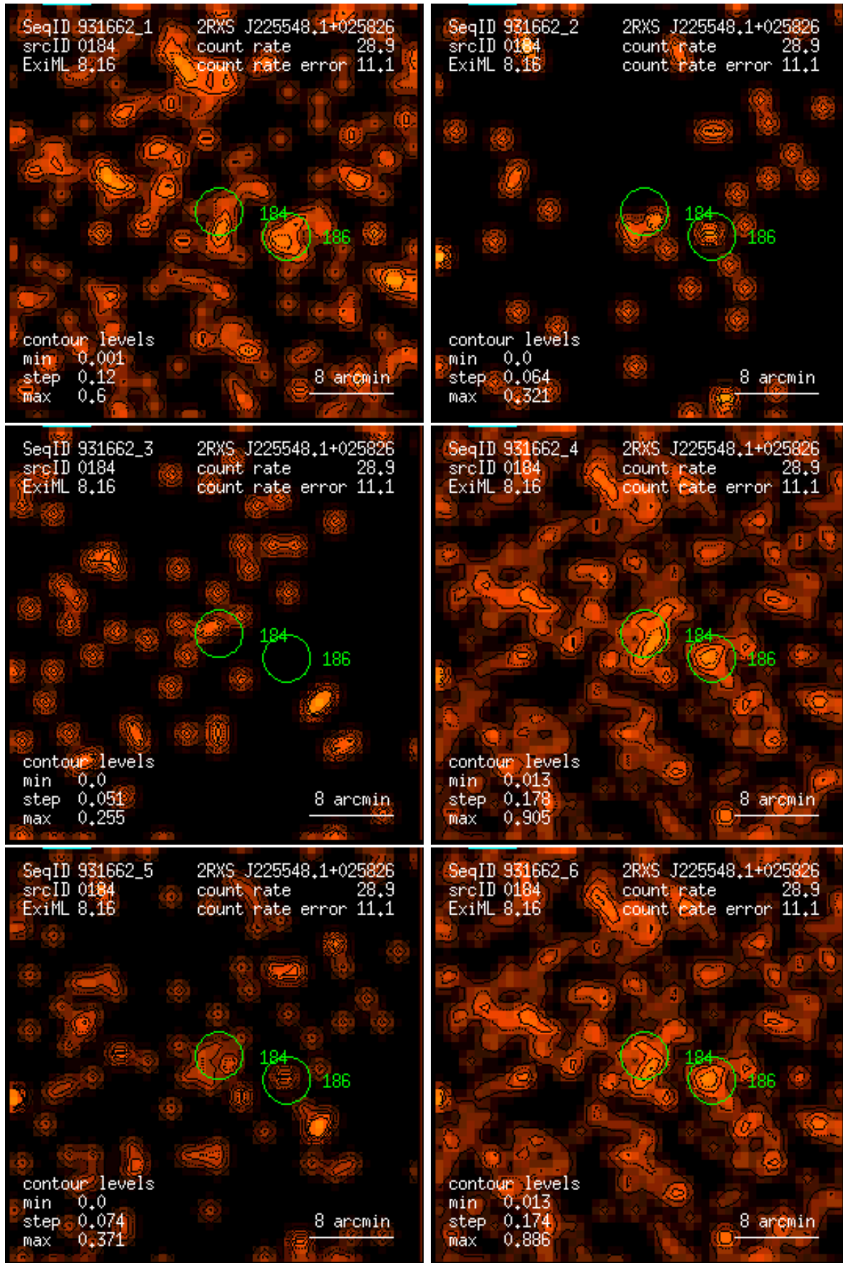
Figure 184: RASS 931662: detection 0184: band rate images, Gaussian filter: (1) PSPC channels 11 – 41, (2) 52 – 90, (3) 91 – 201, (4) 11 – 235, (5) 52 – 201, (6) 11 – 201. Broad band rates in counts/ks. Band rate contour levels in counts/ks/arcmin 2 .
