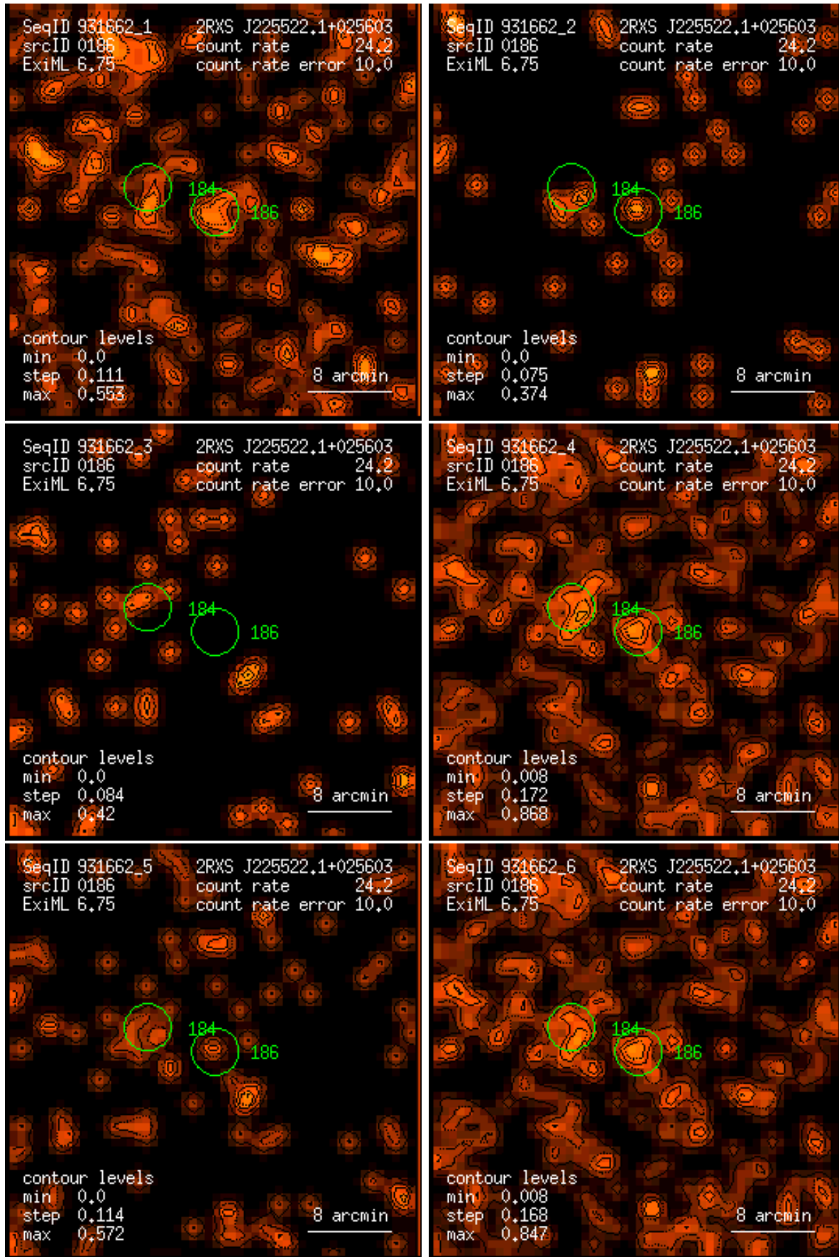
Figure 186: RASS 931662: detection 0186: band rate images, Gaussian filter: (1) PSPC channels 11 – 41, (2) 52 – 90, (3) 91 – 201, (4) 11 – 235, (5) 52 – 201, (6) 11 – 201. Broad band rates in counts/ks. Band rate contour levels in counts/ks/arcmin 2 .
