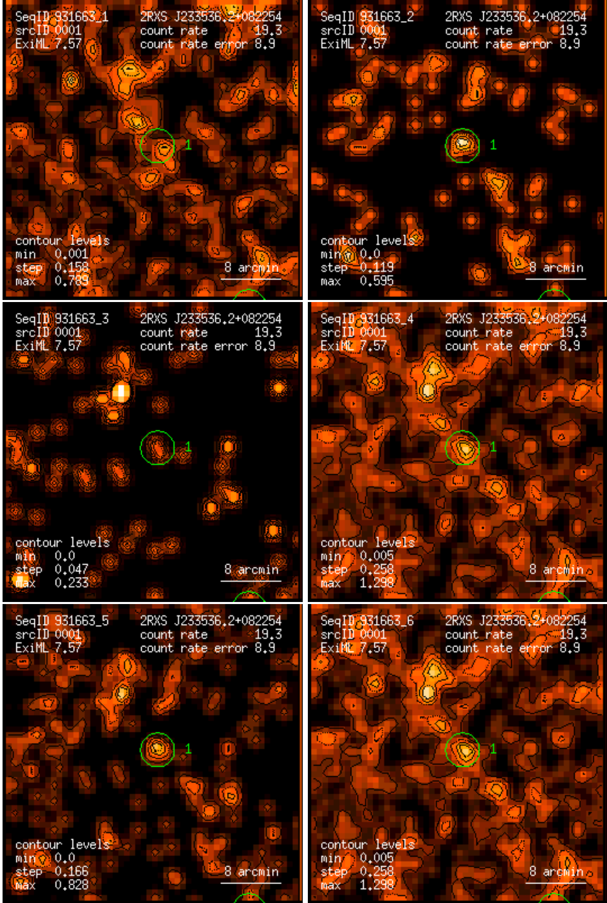
Figure 1: RASS 931663: detection 0001: band rate images, Gaussian filter: (1) PSPC channels 11 – 41, (2) 52 – 90, (3) 91 – 201, (4) 11 – 235, (5) 52 – 201, (6) 11 – 201. Broad band rates in counts/ks. Band rate contour levels in counts/ks/arcmin 2 .
