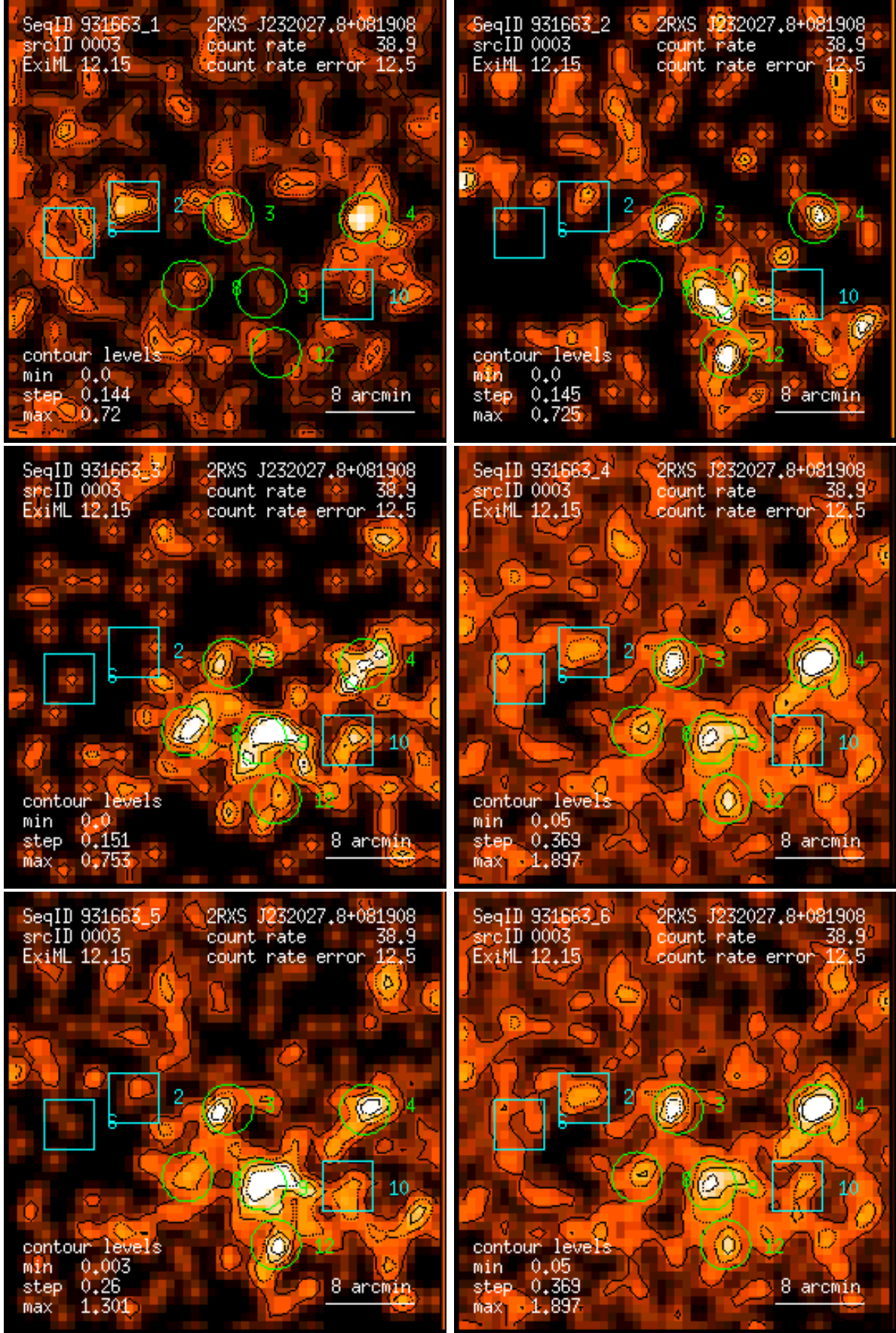
Figure 3: RASS 931663: detection 0003: band rate images, Gaussian filter: (1) PSPC channels 11 – 41, (2) 52 – 90, (3) 91 – 201, (4) 11 – 235, (5) 52 – 201, (6) 11 – 201. Broad band rates in counts/ks. Band rate contour levels in counts/ks/arcmin 2 .
