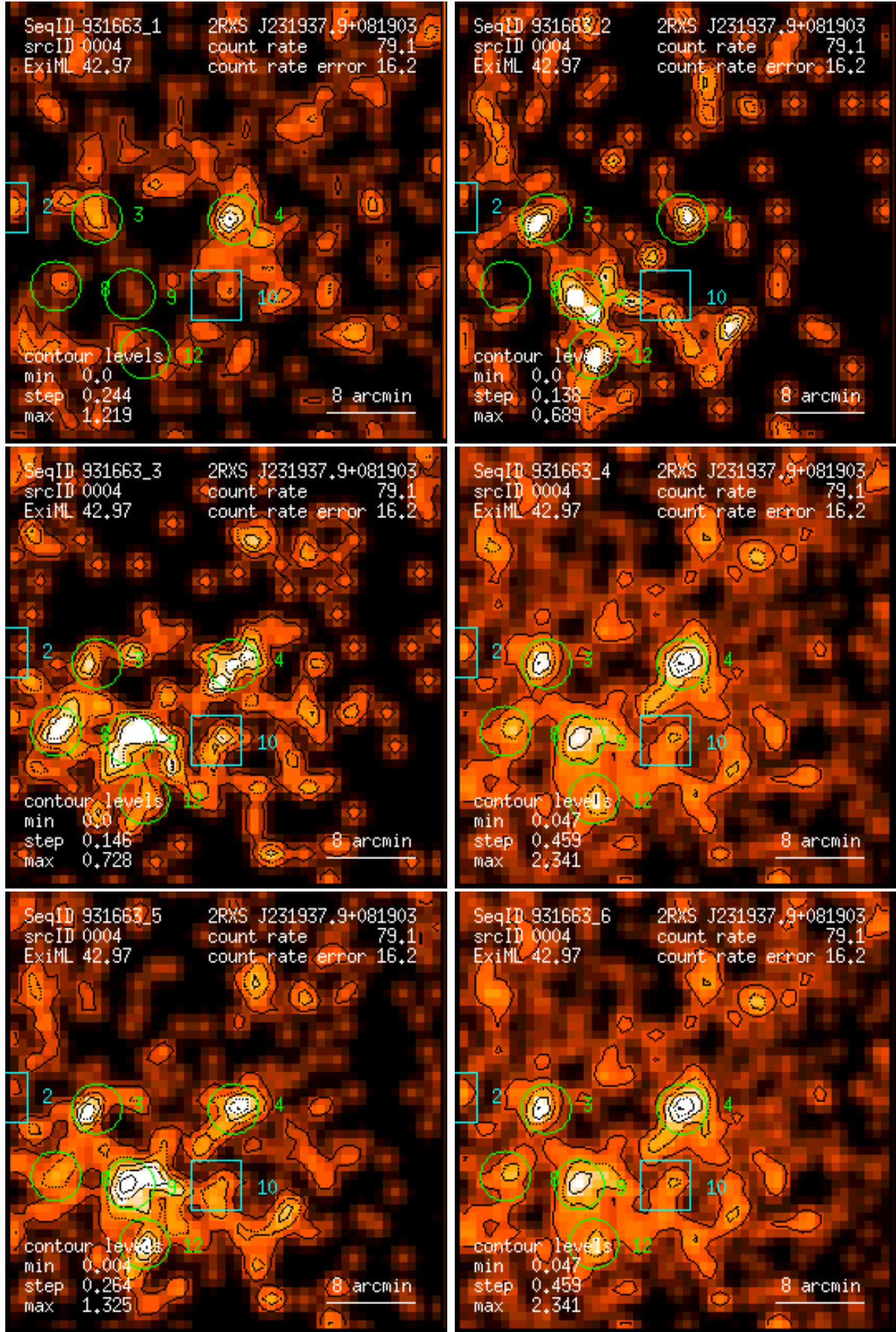
Figure 4: RASS 931663: detection 0004: band rate images, Gaussian filter: (1) PSPC channels 11 – 41, (2) 52 – 90, (3) 91 – 201, (4) 11 – 235, (5) 52 – 201, (6) 11 – 201. Broad band rates in counts/ks. Band rate contour levels in counts/ks/arcmin 2 .
