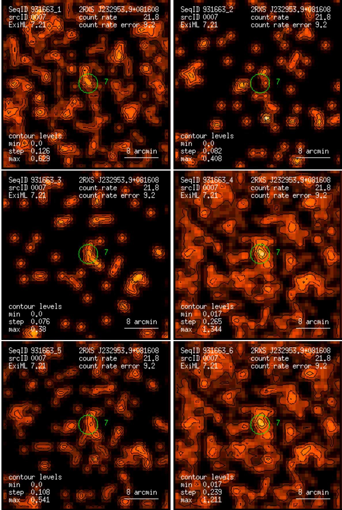
Figure 7: RASS 931663: detection 0007: band rate images, Gaussian filter: (1) PSPC channels 11 – 41, (2) 52 – 90, (3) 91 – 201, (4) 11 – 235, (5) 52 – 201, (6) 11 – 201. Broad band rates in counts/ks. Band rate contour levels in counts/ks/arcmin 2 .
