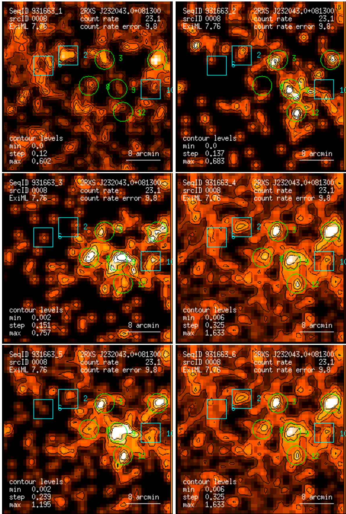
Figure 8: RASS 931663: detection 0008: band rate images, Gaussian filter: (1) PSPC channels 11 – 41, (2) 52 – 90, (3) 91 – 201, (4) 11 – 235, (5) 52 – 201, (6) 11 – 201. Broad band rates in counts/ks. Band rate contour levels in counts/ks/arcmin 2 .
