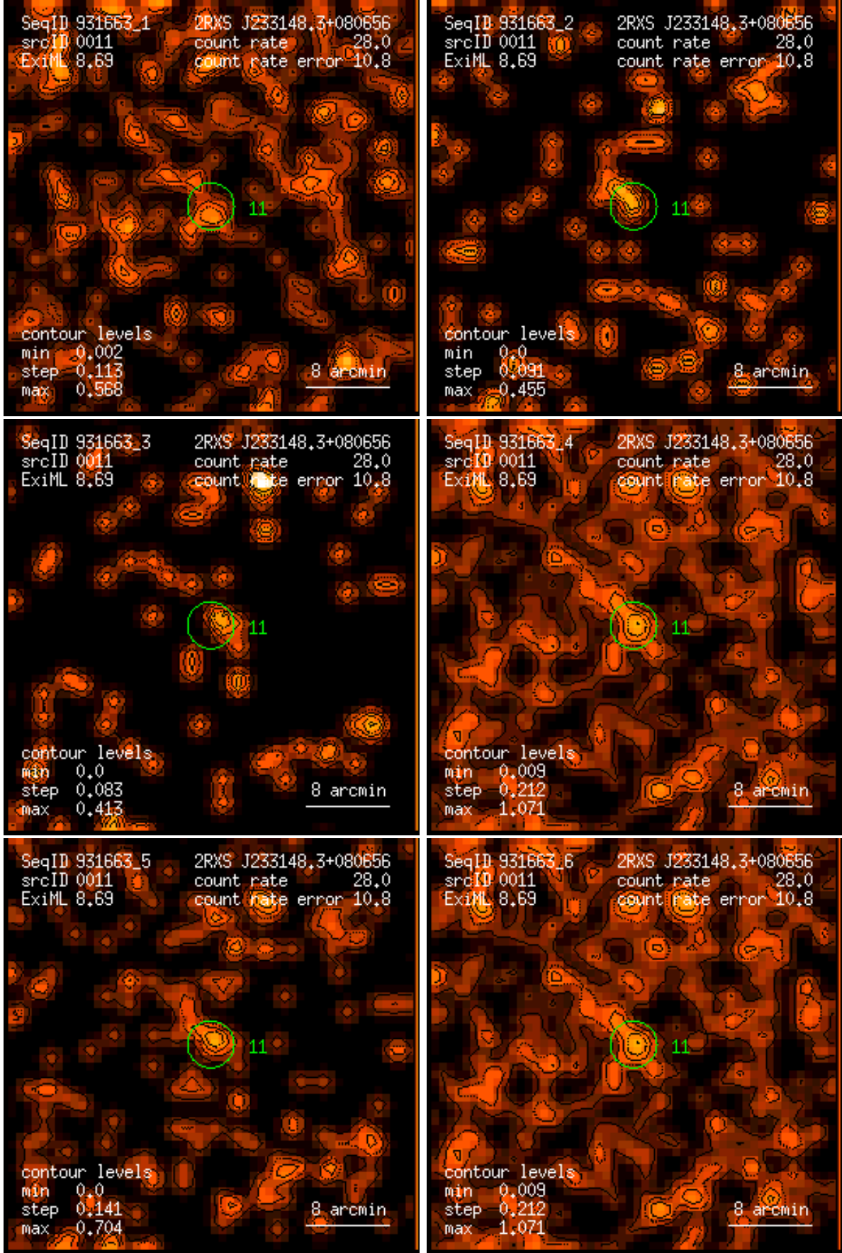
Figure 11: RASS 931663: detection 0011: band rate images, Gaussian filter: (1) PSPC channels 11 – 41, (2) 52 – 90, (3) 91 – 201, (4) 11 – 235, (5) 52 – 201, (6) 11 – 201. Broad band rates in counts/ks. Band rate contour levels in counts/ks/arcmin 2 .
