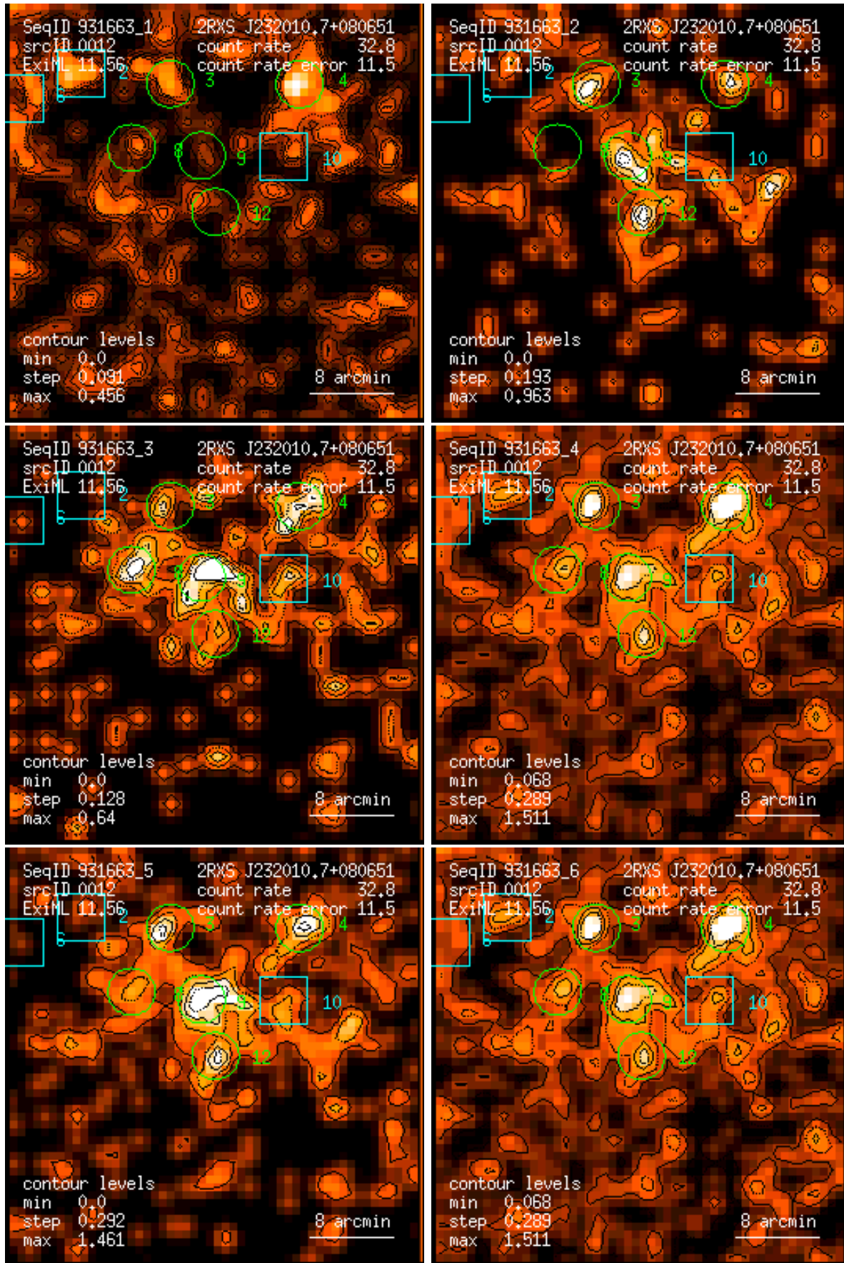
Figure 12: RASS 931663: detection 0012: band rate images, Gaussian filter: (1) PSPC channels 11 – 41, (2) 52 – 90, (3) 91 – 201, (4) 11 – 235, (5) 52 – 201, (6) 11 – 201. Broad band rates in counts/ks. Band rate contour levels in counts/ks/arcmin 2 .
