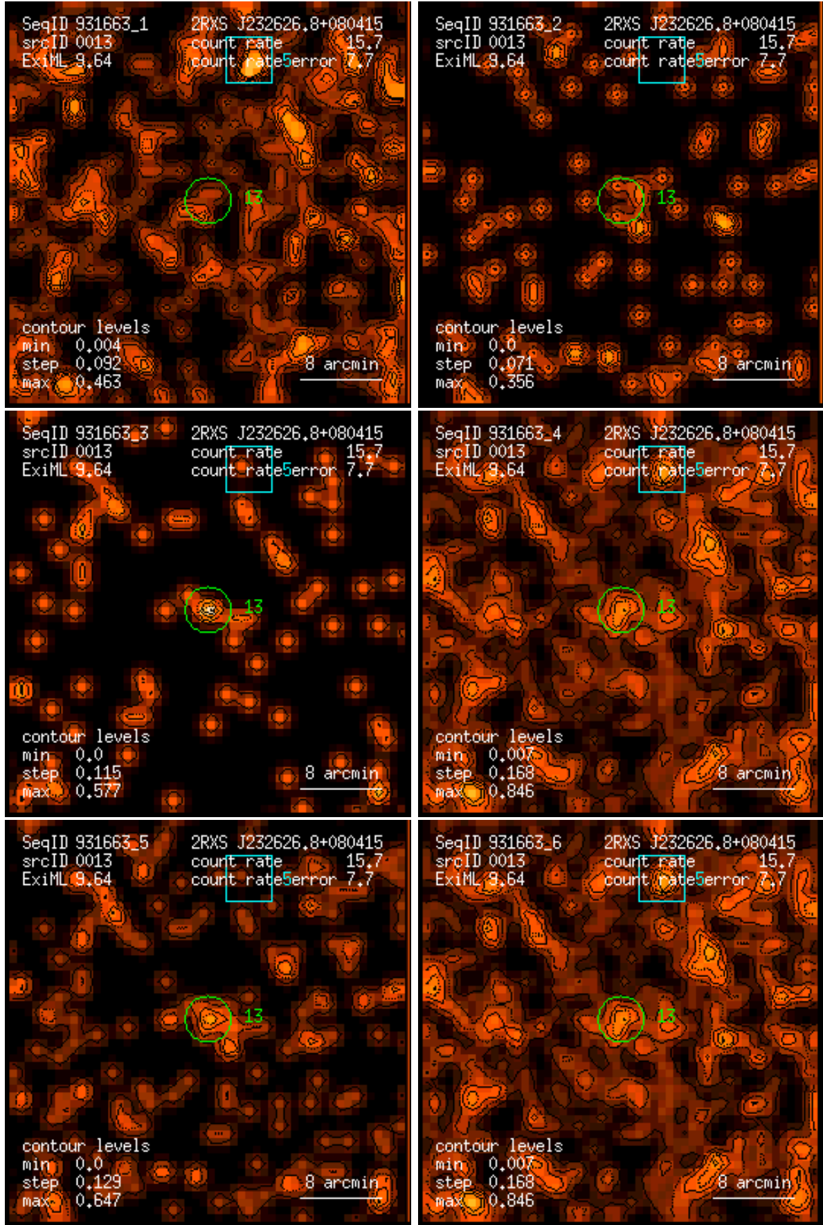
Figure 13: RASS 931663: detection 0013: band rate images, Gaussian filter: (1) PSPC channels 11 – 41, (2) 52 – 90, (3) 91 – 201, (4) 11 – 235, (5) 52 – 201, (6) 11 – 201. Broad band rates in counts/ks. Band rate contour levels in counts/ks/arcmin 2 .
