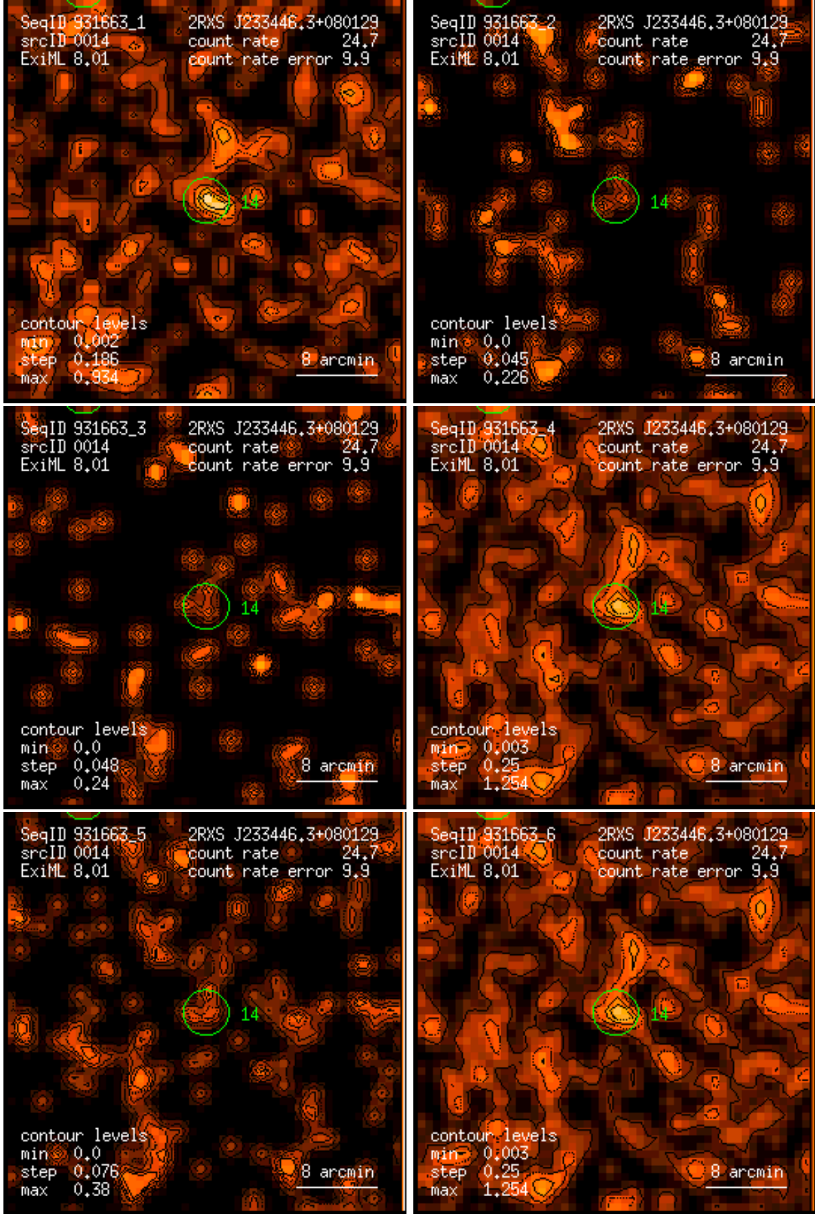
Figure 14: RASS 931663: detection 0014: band rate images, Gaussian filter: (1) PSPC channels 11 – 41, (2) 52 – 90, (3) 91 – 201, (4) 11 – 235, (5) 52 – 201, (6) 11 – 201. Broad band rates in counts/ks. Band rate contour levels in counts/ks/arcmin 2 .
