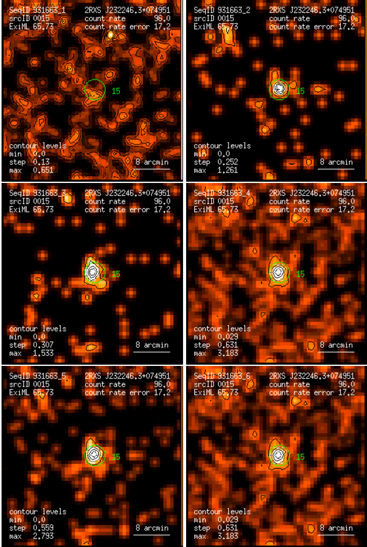
Figure 15: RASS 931663: detection 0015: band rate images, Gaussian filter: (1) PSPC channels 11 – 41, (2) 52 – 90, (3) 91 – 201, (4) 11 – 235, (5) 52 – 201, (6) 11 – 201. Broad band rates in counts/ks. Band rate contour levels in counts/ks/arcmin 2 .
