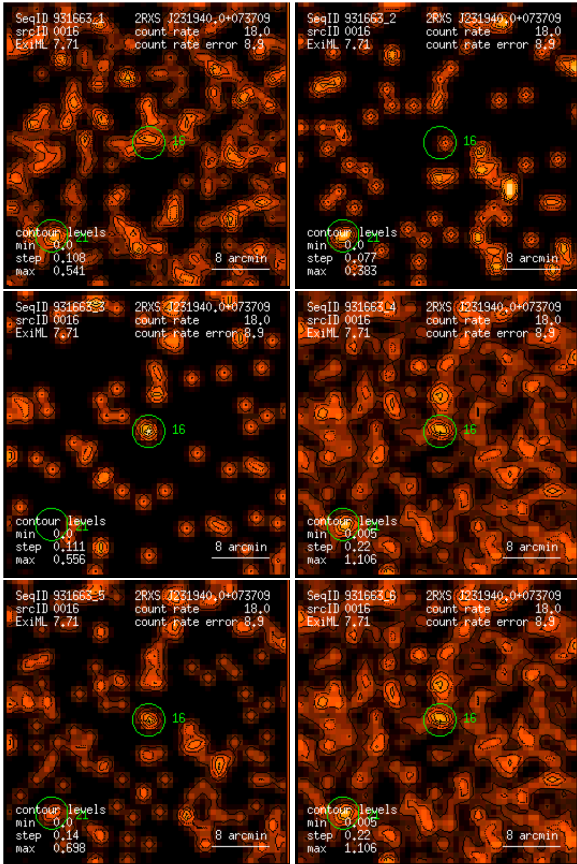
Figure 16: RASS 931663: detection 0016: band rate images, Gaussian filter: (1) PSPC channels 11 – 41, (2) 52 – 90, (3) 91 – 201, (4) 11 – 235, (5) 52 – 201, (6) 11 – 201. Broad band rates in counts/ks. Band rate contour levels in counts/ks/arcmin 2 .
