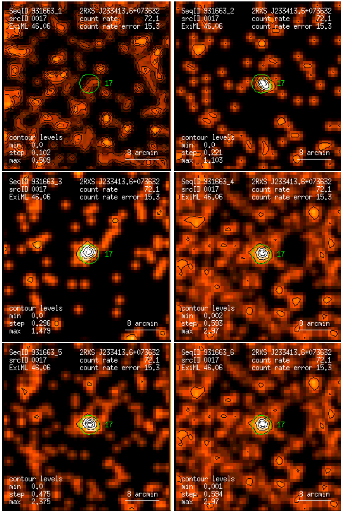
Figure 17: RASS 931663: detection 0017: band rate images, Gaussian filter: (1) PSPC channels 11 – 41, (2) 52 – 90, (3) 91 – 201, (4) 11 – 235, (5) 52 – 201, (6) 11 – 201. Broad band rates in counts/ks. Band rate contour levels in counts/ks/arcmin 2 .
