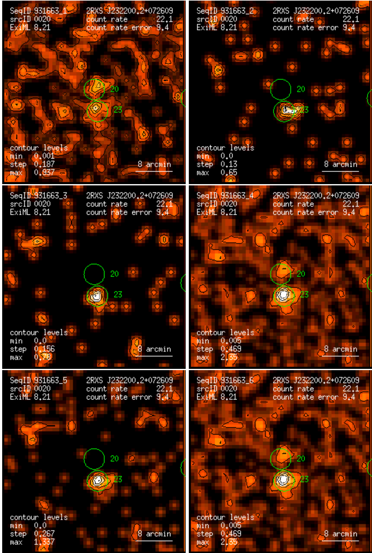
Figure 20: RASS 931663: detection 0020: band rate images, Gaussian filter: (1) PSPC channels 11 – 41, (2) 52 – 90, (3) 91 – 201, (4) 11 – 235, (5) 52 – 201, (6) 11 – 201. Broad band rates in counts/ks. Band rate contour levels in counts/ks/arcmin 2 .
