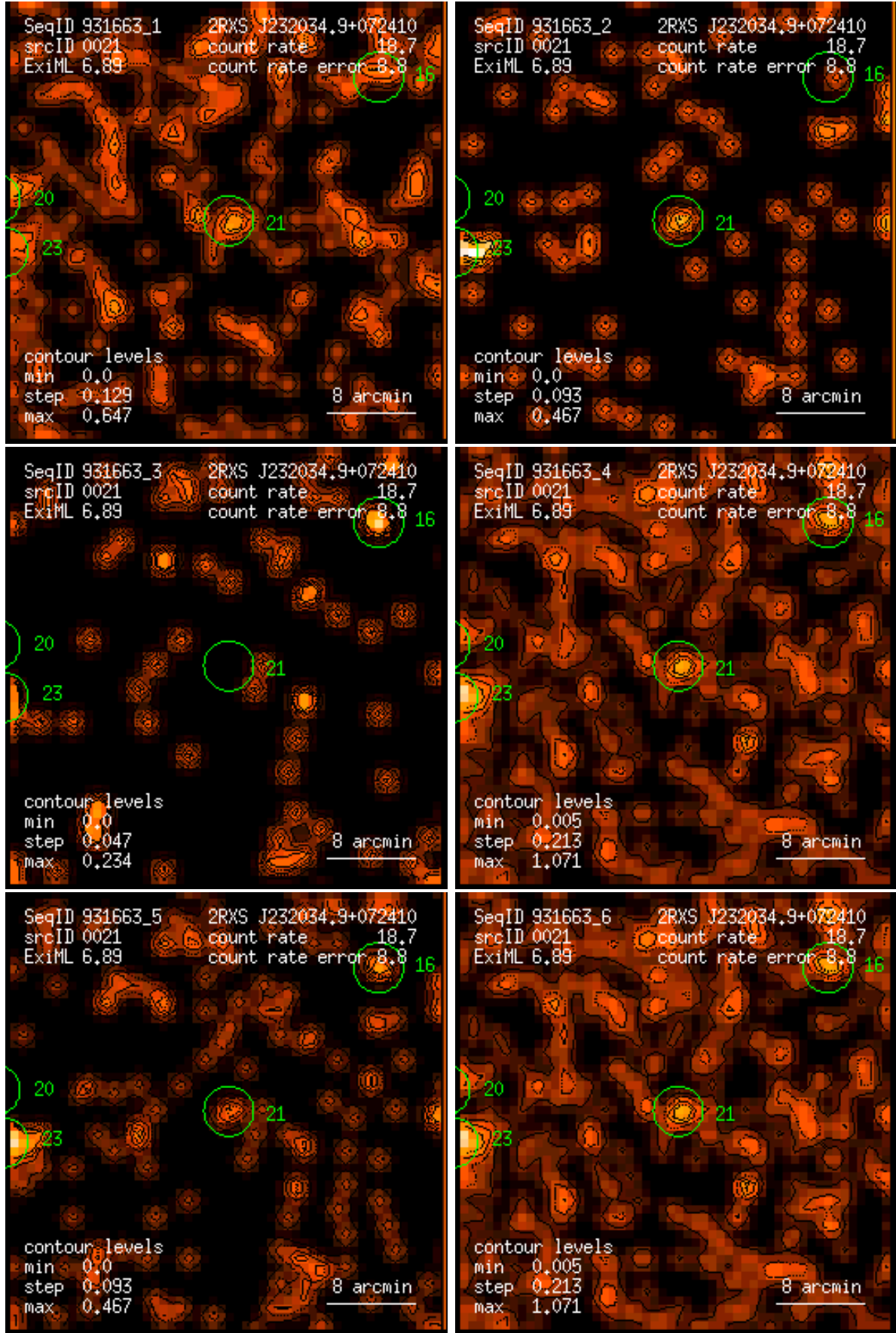
Figure 21: RASS 931663: detection 0021: band rate images, Gaussian filter: (1) PSPC channels 11 – 41, (2) 52 – 90, (3) 91 – 201, (4) 11 – 235, (5) 52 – 201, (6) 11 – 201. Broad band rates in counts/ks. Band rate contour levels in counts/ks/arcmin 2 .
