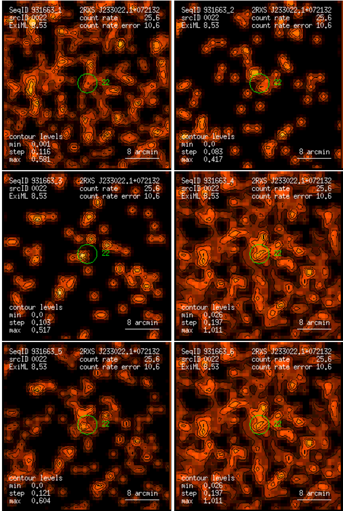
Figure 22: RASS 931663: detection 0022: band rate images, Gaussian filter: (1) PSPC channels 11 – 41, (2) 52 – 90, (3) 91 – 201, (4) 11 – 235, (5) 52 – 201, (6) 11 – 201. Broad band rates in counts/ks. Band rate contour levels in counts/ks/arcmin 2 .
