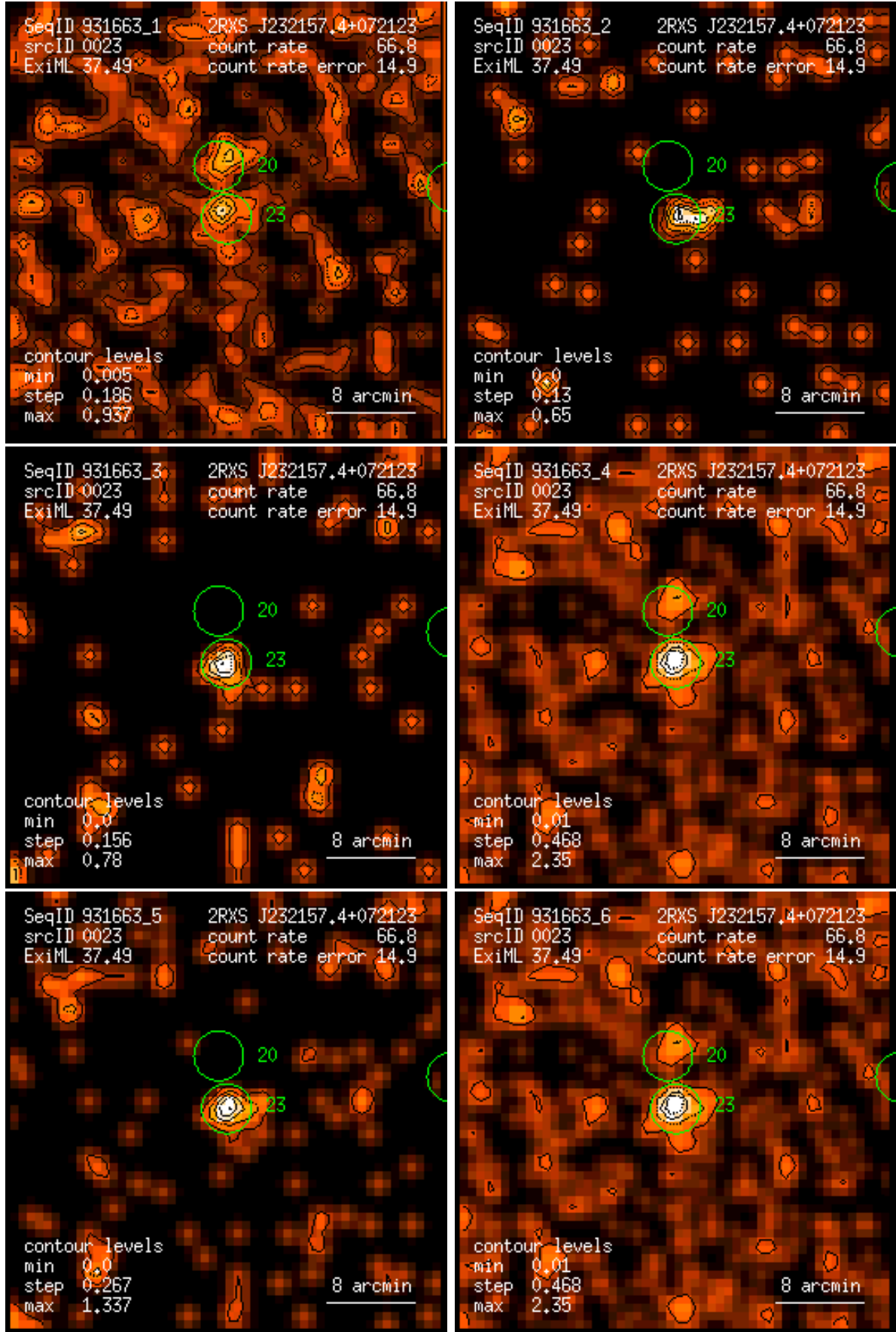
Figure 23: RASS 931663: detection 0023: band rate images, Gaussian filter: (1) PSPC channels 11 – 41, (2) 52 – 90, (3) 91 – 201, (4) 11 – 235, (5) 52 – 201, (6) 11 – 201. Broad band rates in counts/ks. Band rate contour levels in counts/ks/arcmin 2 .
