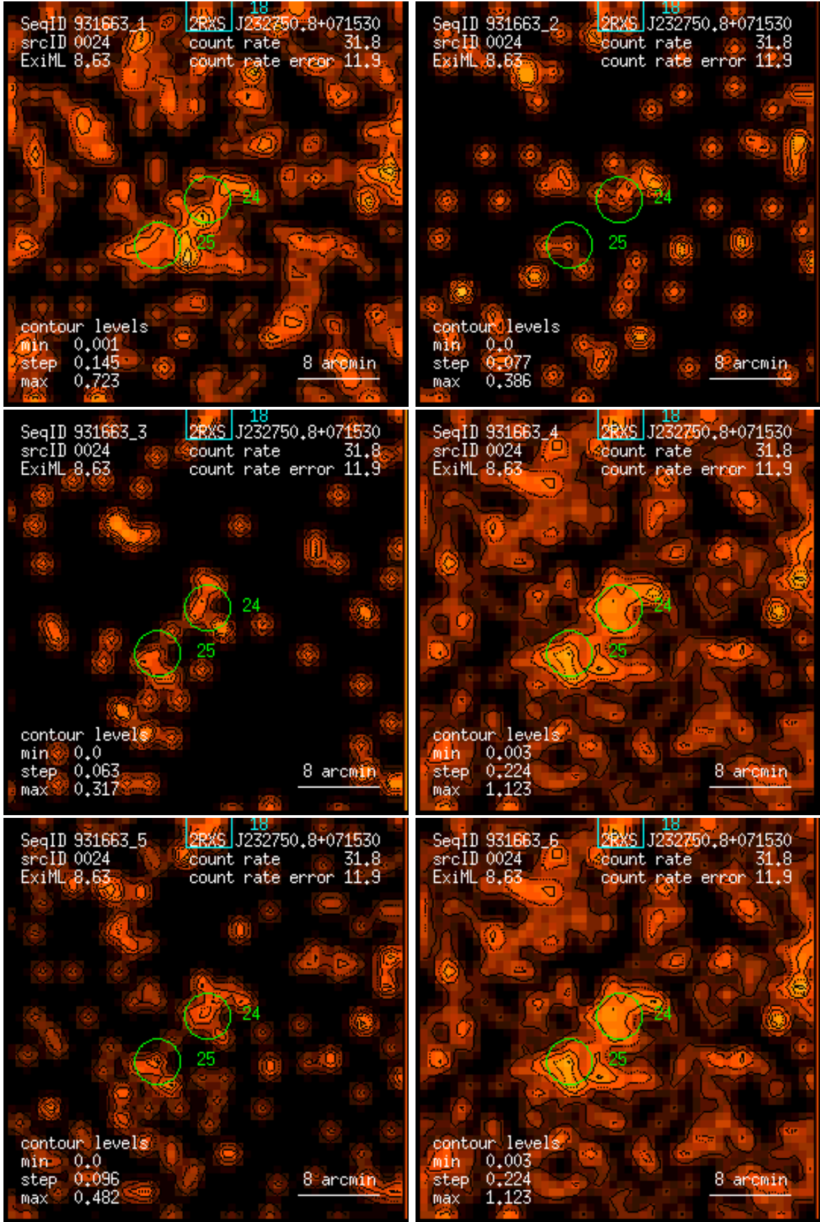
Figure 24: RASS 931663: detection 0024: band rate images, Gaussian filter: (1) PSPC channels 11 – 41, (2) 52 – 90, (3) 91 – 201, (4) 11 – 235, (5) 52 – 201, (6) 11 – 201. Broad band rates in counts/ks. Band rate contour levels in counts/ks/arcmin 2 .
