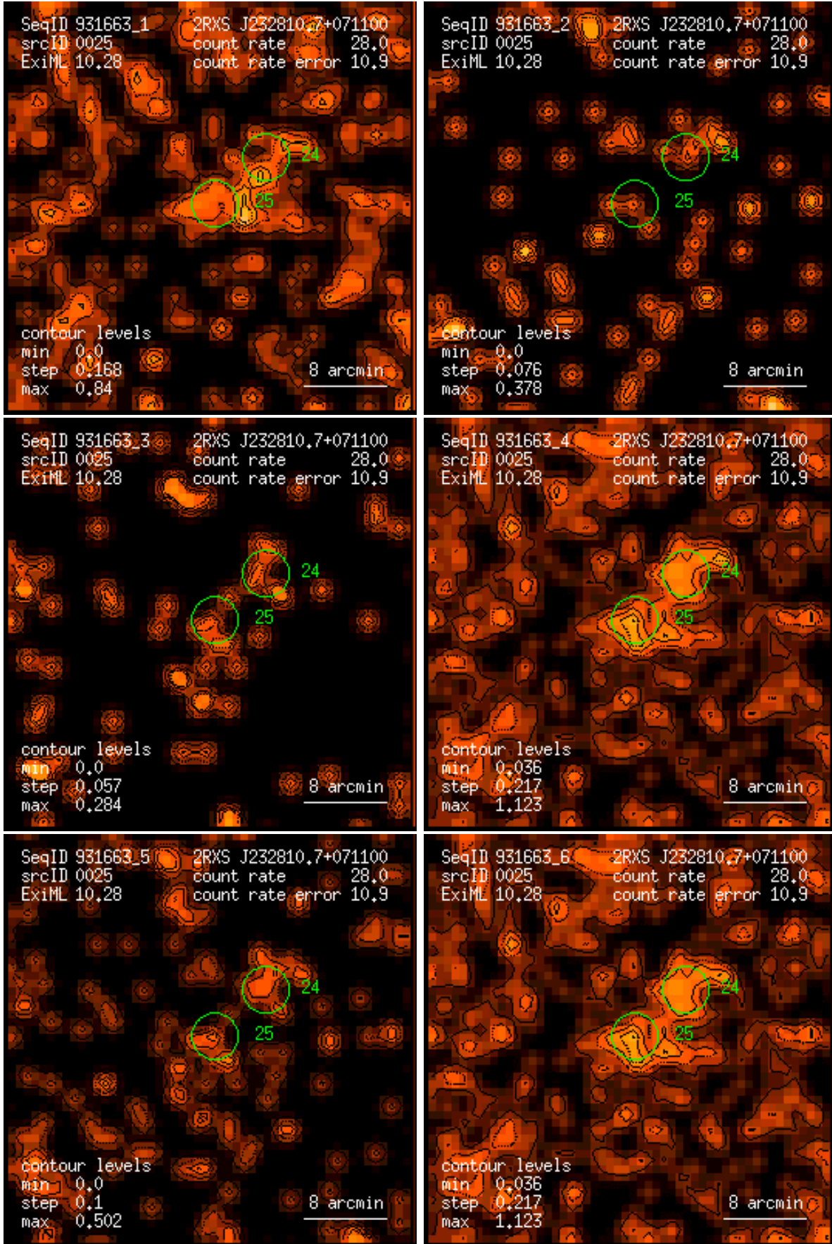
Figure 25: RASS 931663: detection 0025: band rate images, Gaussian filter: (1) PSPC channels 11 – 41, (2) 52 – 90, (3) 91 – 201, (4) 11 – 235, (5) 52 – 201, (6) 11 – 201. Broad band rates in counts/ks. Band rate contour levels in counts/ks/arcmin 2 .
