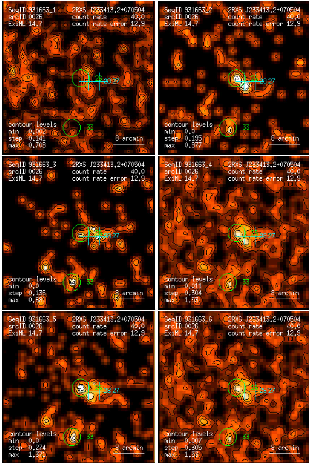
Figure 26: RASS 931663: detection 0026: band rate images, Gaussian filter: (1) PSPC channels 11 – 41, (2) 52 – 90, (3) 91 – 201, (4) 11 – 235, (5) 52 – 201, (6) 11 – 201. Broad band rates in counts/ks. Band rate contour levels in counts/ks/arcmin 2 .
