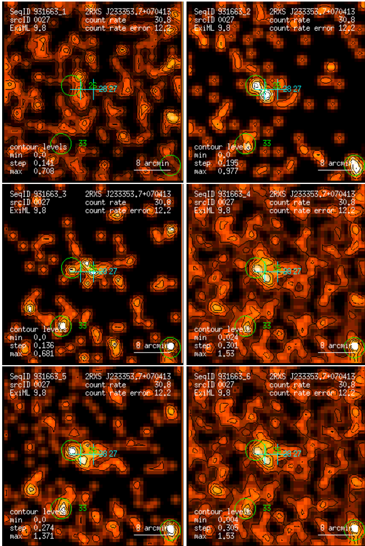
Figure 27: RASS 931663: detection 0027: band rate images, Gaussian filter: (1) PSPC channels 11 – 41, (2) 52 – 90, (3) 91 – 201, (4) 11 – 235, (5) 52 – 201, (6) 11 – 201. Broad band rates in counts/ks. Band rate contour levels in counts/ks/arcmin 2 .
