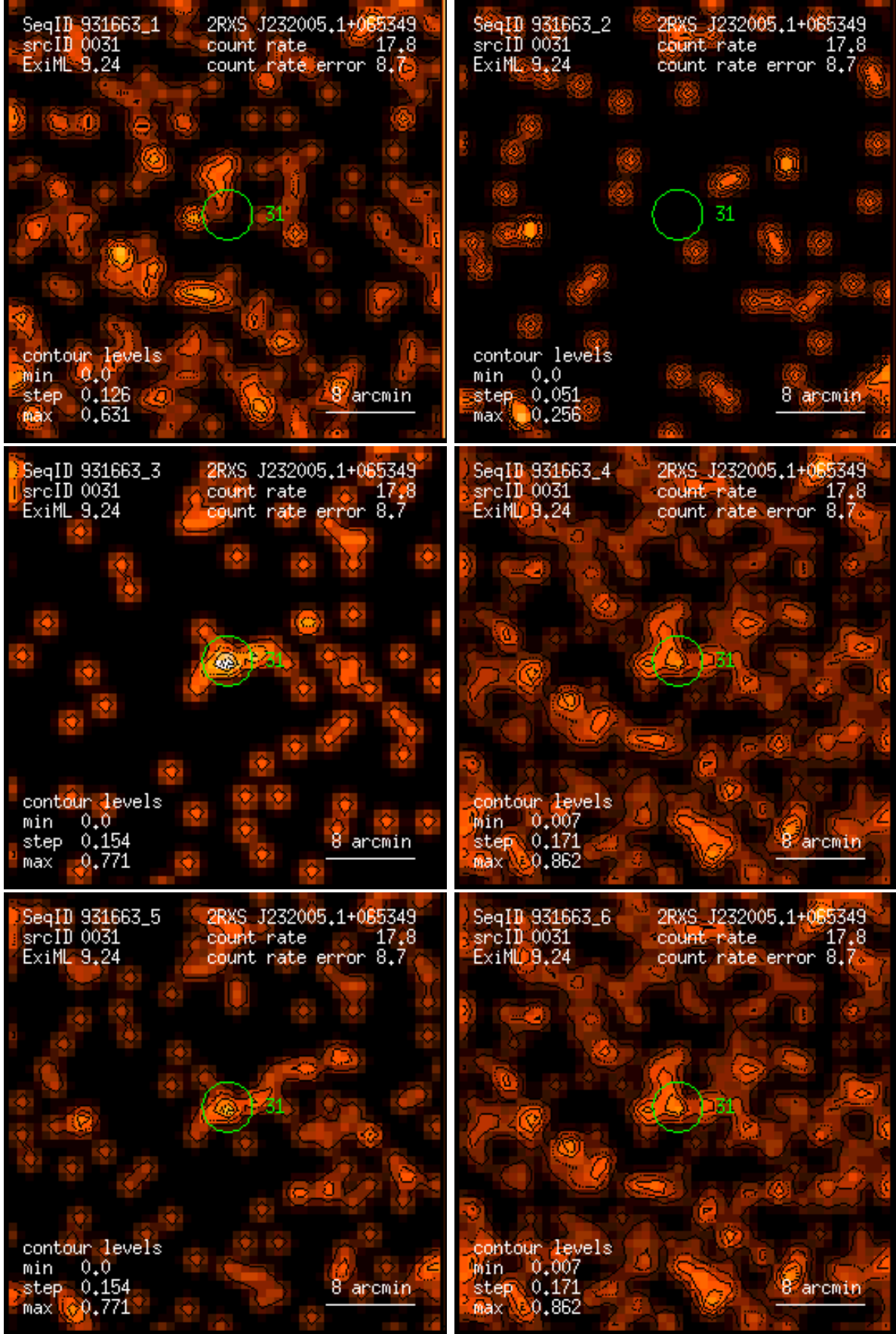
Figure 31: RASS 931663: detection 0031: band rate images, Gaussian filter: (1) PSPC channels 11 – 41, (2) 52 – 90, (3) 91 – 201, (4) 11 – 235, (5) 52 – 201, (6) 11 – 201. Broad band rates in counts/ks. Band rate contour levels in counts/ks/arcmin 2 .
